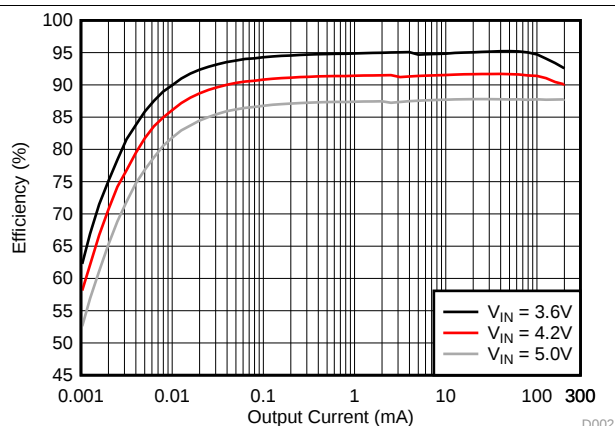
Figure 4. TPS82740A Efficiency V_{OUT} = 2.1\text{V}
