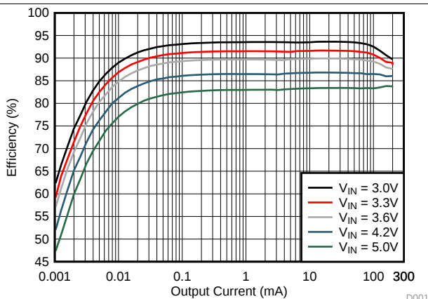
Figure 3. TPS82740A Efficiency V_{OUT} = 1.8\text{V}
