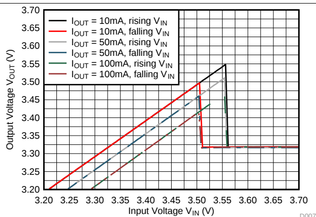
Figure 20. TPS82740B 100% Mode Transition V_{OUT} = 3.3V
