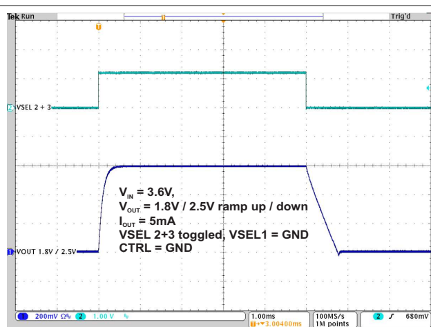
Figure 44. TPS82740A Dynamic Output Voltage Scaling: V_{OUT} = 1.8V / 2.5V
