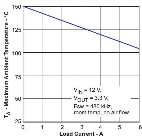
图 8-15. Maximum Ambient Temperature vs Load Current
