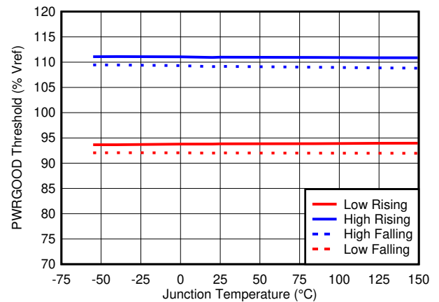
图 6-12. PWRGD Threshold vs Temperature
