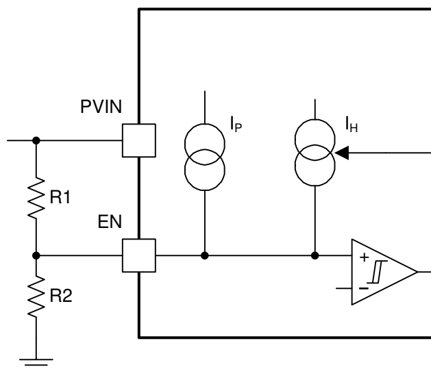
图 7-2. Adjustable PVIN Undervoltage Lockout, VIN ≥ 4.5 V
