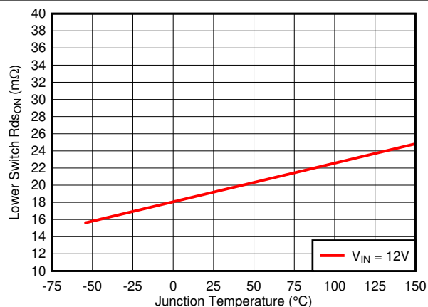
图 6-2. Low-Side R_{DS(on)} vs Temperature
