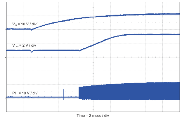
图 8-5. Start-Up With PRE-BIAS
