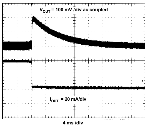
Figure 47. Unload Transient
