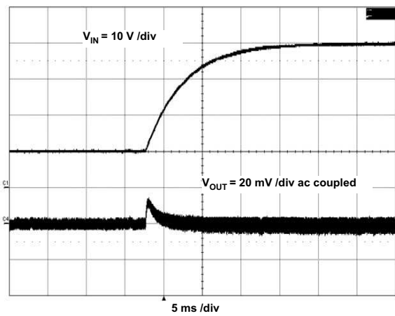
Figure 29. Line Transient
