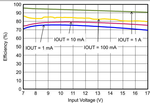
图 11. Efficiency With 1.25 MHz
