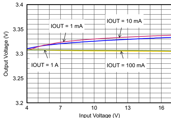
图 23. Output Voltage Accuracy (Line Regulation)
