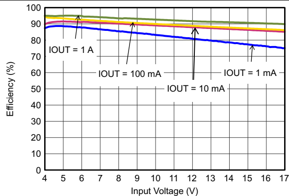
图 13. Efficiency With 2.5 MHz
