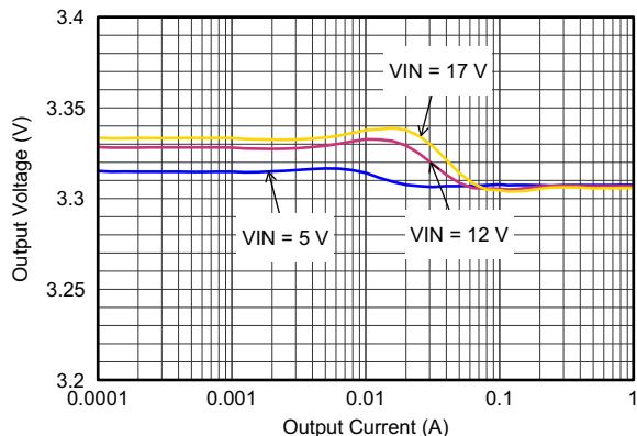
图 22. Output Voltage Accuracy (Load Regulation)
