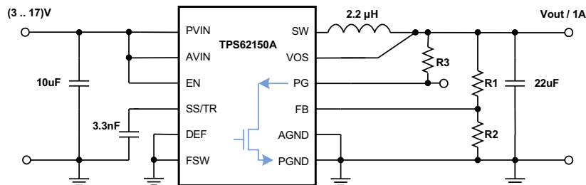
图 45. Discharge V_{OUT} Through PG Pin with TPS62150A
