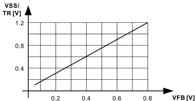
图 8. Voltage Tracking Relationship
