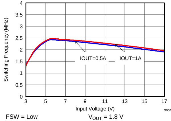
图 28. Switching Frequency vs Input Voltage
