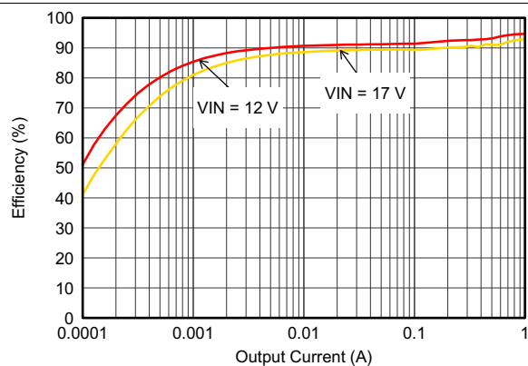
图 10. Efficiency With 1.25 MHz
