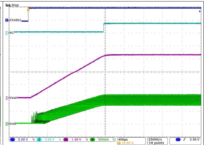
图 41. Start-Up Into 1 A
