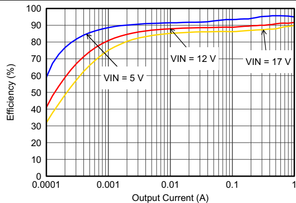
图 12. Efficiency With 2.5 MHz
