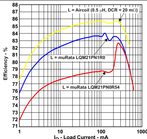
Figure 7. Efficiency vs Load Current, V OUT = 1.2 V
