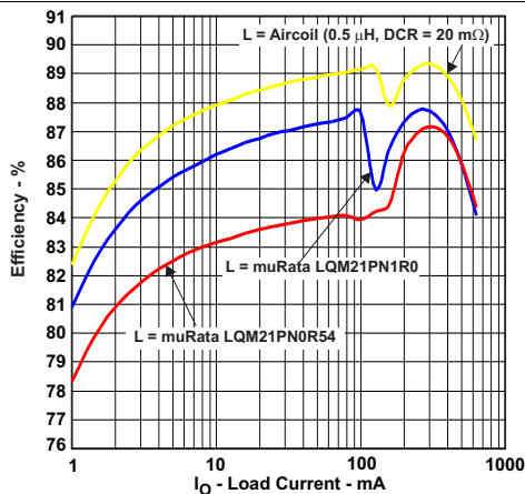
Figure 8. Efficiency vs Load Current, V OUT = 1.82 V, PWM/PFM Operation
