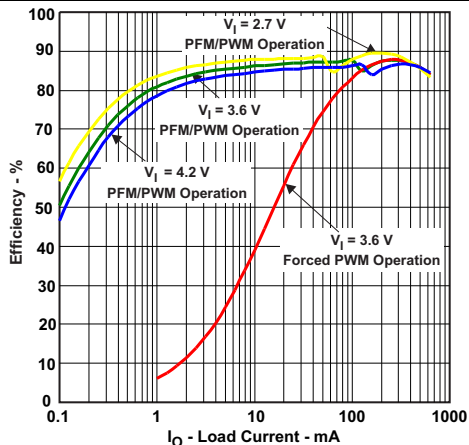
Figure 6. Efficiency vs Load Current, V OUT = 1.82 V
