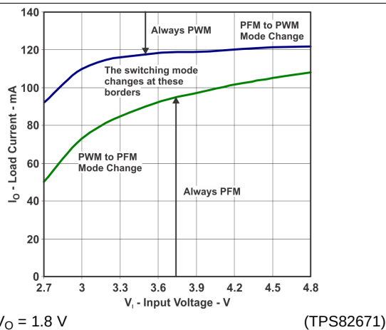
Figure 39. PFM/PWM Boundaries
