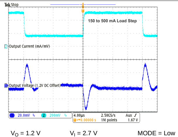
Figure 36. Load Transient Response in PFM/PWM Operation
