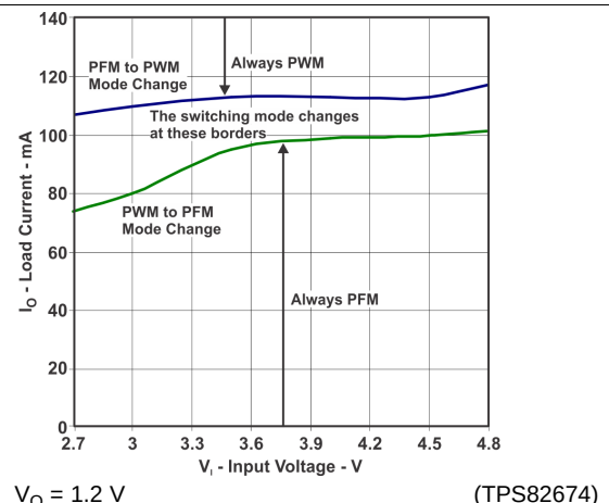
Figure 40. PFM/PWM Boundaries
