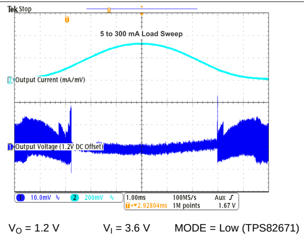
Figure 38. AC Load Transient Response
