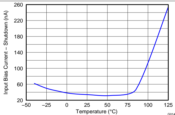
Figure 15. Input Bias Current vs Temperature, Shutdown
