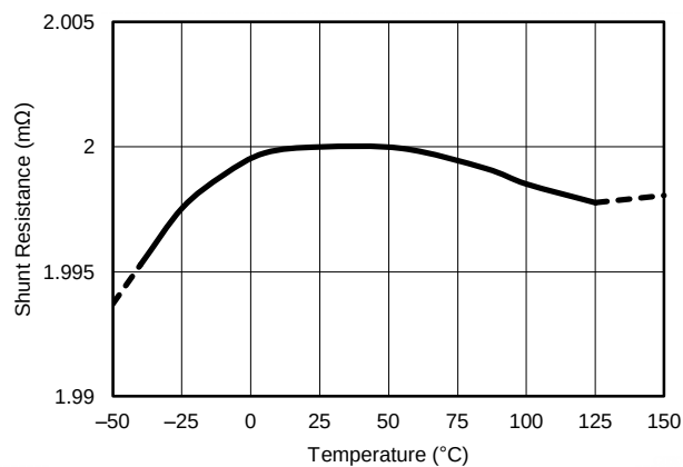
Figure 32. Sensing Resistor vs Temperature
