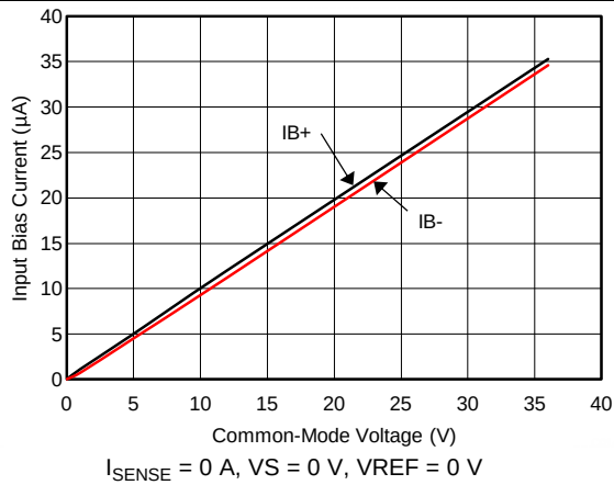
Figure 21. Input Bias Current vs Common-Mode Voltage ( V_S = 0\text{ V} )
