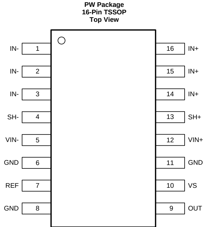
Pin Functions
