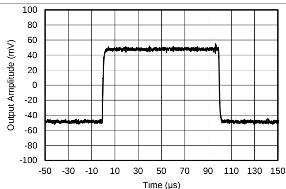
图 40. Small-Signal Response
