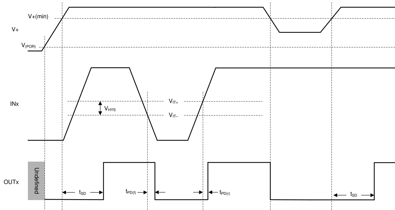
Figure 1. Timing Diagram
