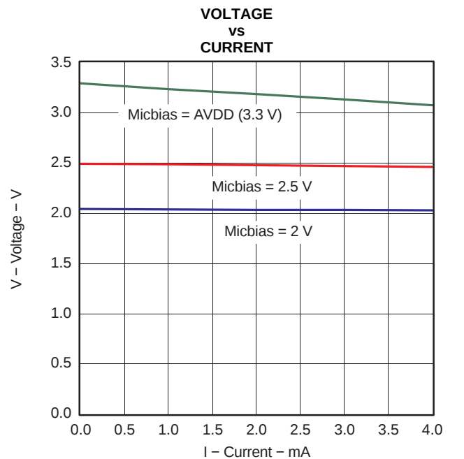
Figure 4-14. MICBIAS
