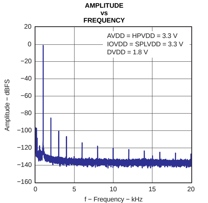
Figure 4-13. FFT – Line-In Bypass to Headphone Output
