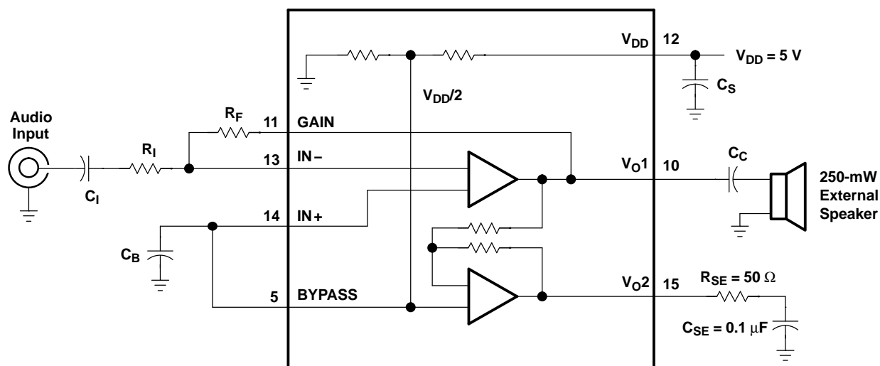
Figure 38. Single-Ended Mode
