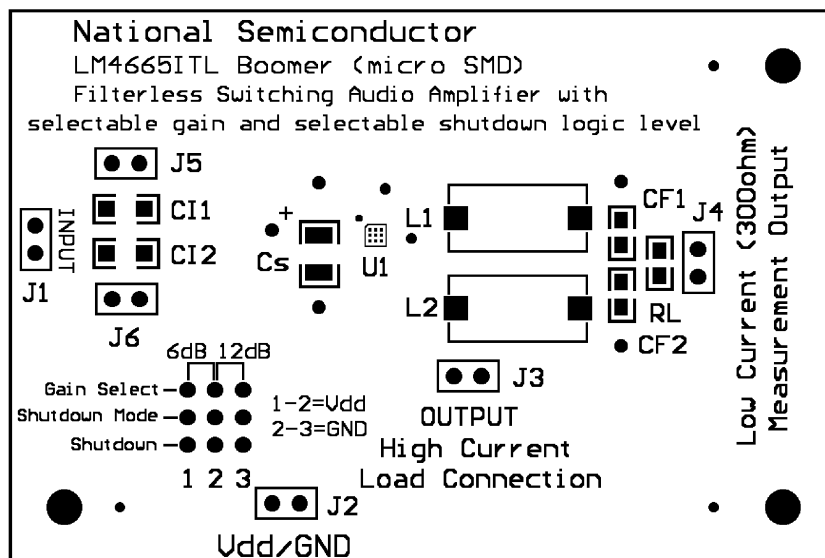
Figure 45. Silk Screen
