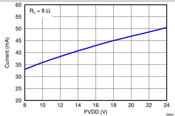
With LC Filter as Shown on EVM Figure 26. Idle Current Draw vs PVDD
