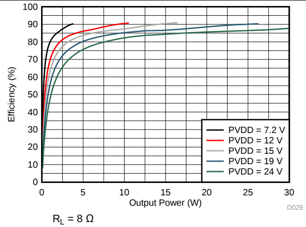
图 32. Efficiency vs Output Power
