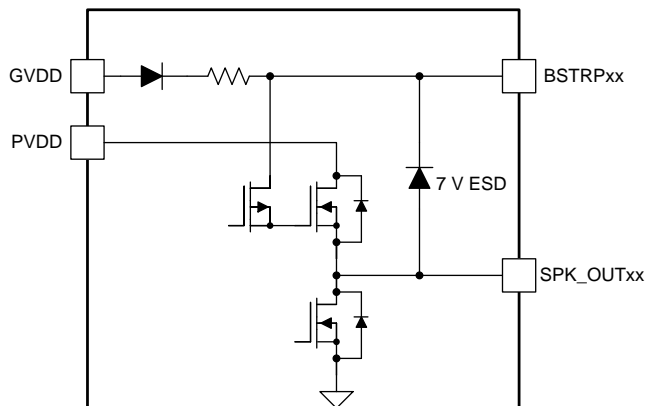
Figure 3. BSTRPx Pins
