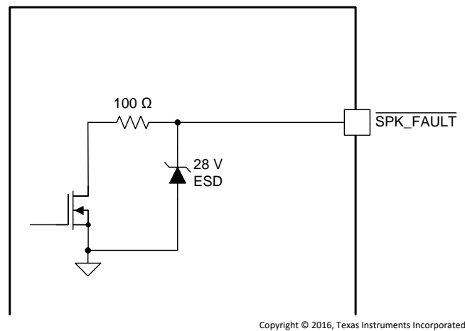
Figure 16. \overline{\text{SPK\_FAULT}} Pin
