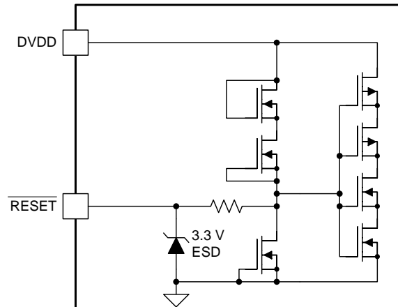
Copyright © 2016, Texas Instruments Incorporated Figure 17. RESET Pin
