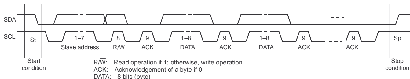
Figure 77. Packet Protocol
