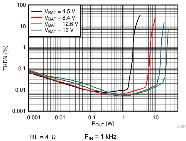
图 6-1. THD+N vs Output Power
