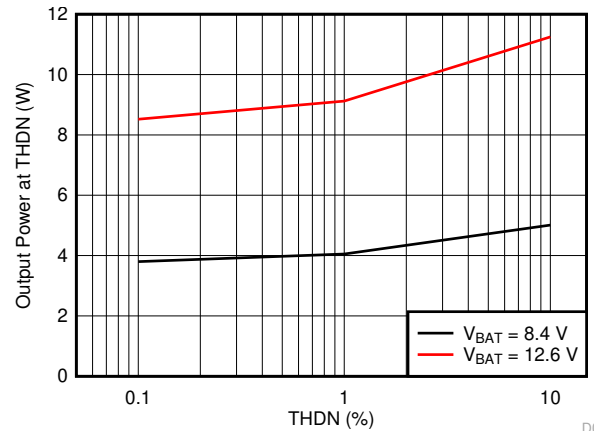
图 6-12. Max Output Power vs THD+N
