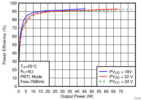
图 6-33. Efficiency vs Output Power
