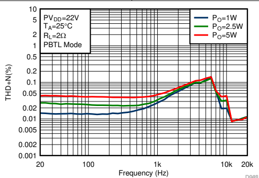
图 6-53. THD+N vs Frequency
