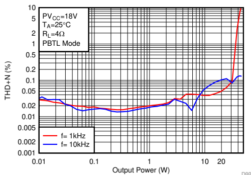
图 6-38. THD+N vs Output Power
