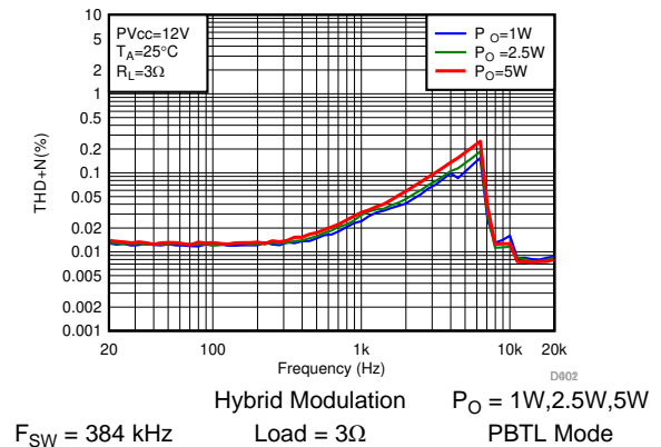
图 27. THD+N vs Frequency-PBTTL
