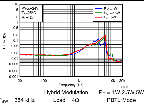
图 30. THD+N vs Frequency-PBTTL
