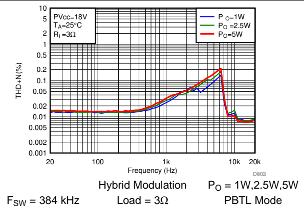
图 29. THD+N vs Frequency-PBTTL
