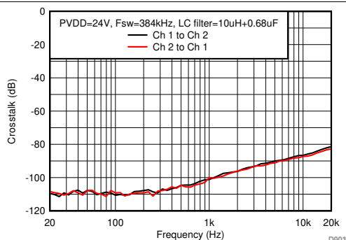
PVDD=24V Hybrid Modulation F SW = 384 kHz Load = 6Ω BTL Mode
