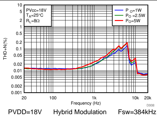
图 164. THD+N vs Frequency
