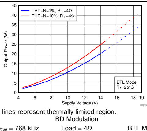
图 60. Output Power vs Supply Voltage
