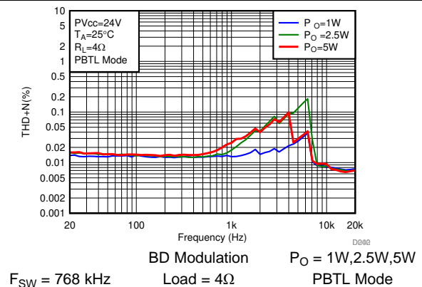
图 77. THD+N vs Frequency-PBTB
