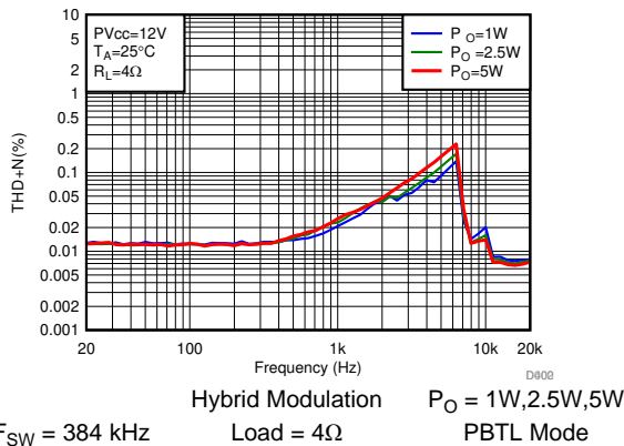
图 26. THD+N vs Frequency-PBTTL
