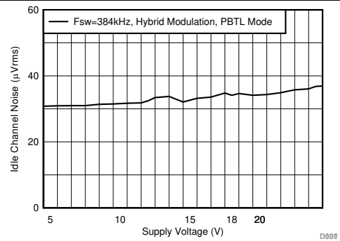
图 39. Idle Channel Noise vs Supply Voltage
