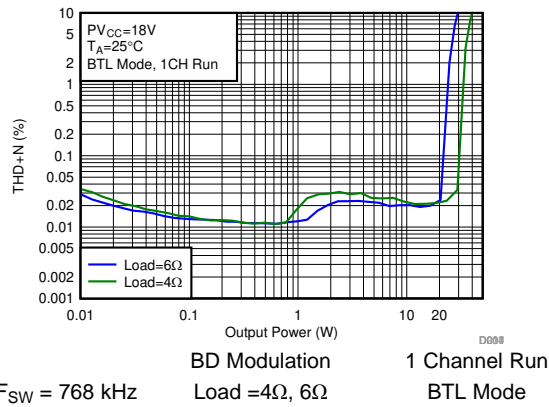
图 57. THD+N vs Output Power-BTL
