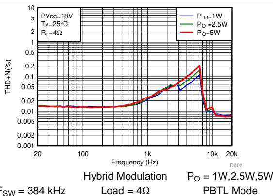
图 28. THD+N vs Frequency-PBTTL
