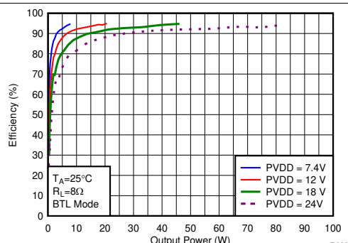
Hybrid Modulation F SW = 384 kHz Load = 8Ω BTL Mode
