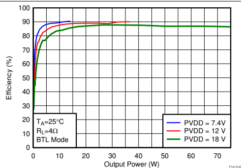
Hybrid Modulation F SW = 384 kHz Load = 4Ω BTL Mode
