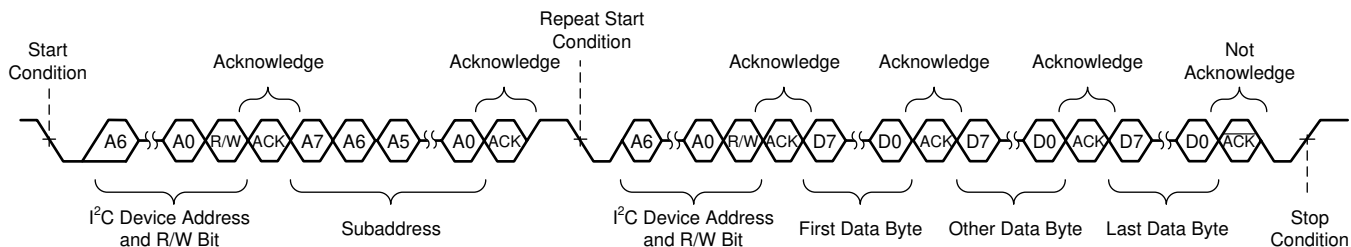
图 102. Sequential Read Transfer
