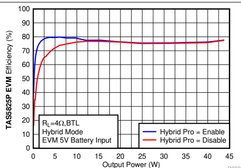
Hybrid Modulation F SW = 384 kHz 5V Battery Input Default PPC3 Setting Load=4Ω, BTL 5V~16V Boost (-5.5dB AGAIN)
