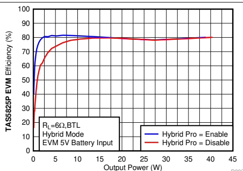
Hybrid Modulation F SW = 384 kHz 5V Battery Input Default PPC3 Setting Load=6Ω, BTL 5V~16V Boost (-5.5dB AGAIN)
