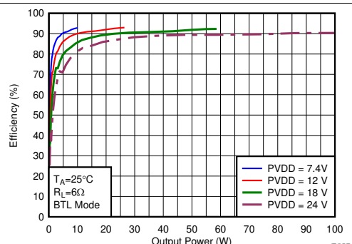
Hybrid Modulation F SW = 384 kHz Load = 6Ω BTL Mode
