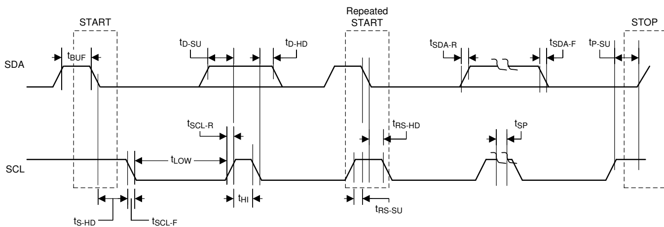
图 89. I 2 C Communication Port Timing Diagram
