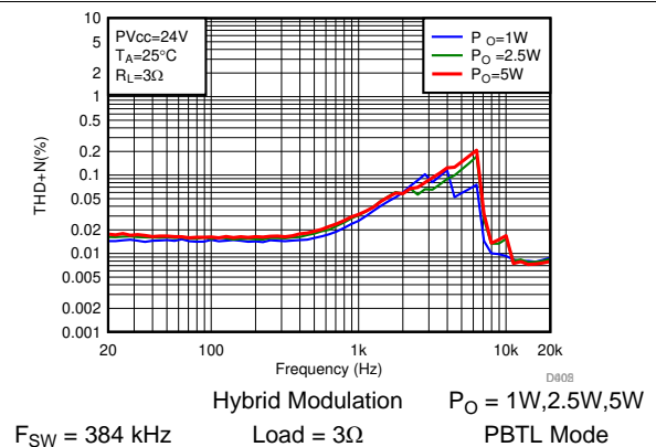
图 31. THD+N vs Frequency-PBTTL
