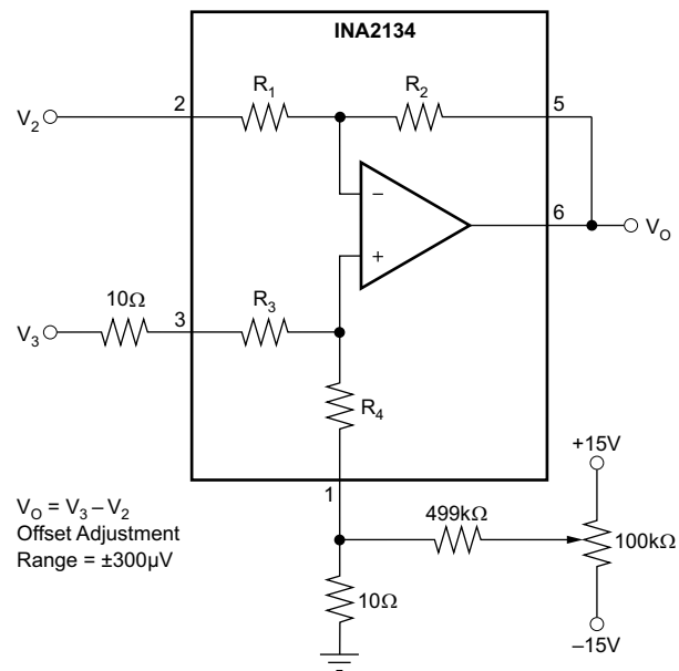
Figure 3. Offset Adjustment
