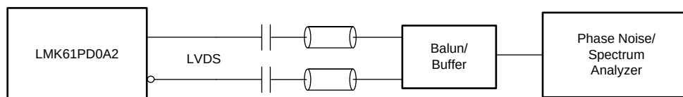
Figure 11. LVDS Output AC Configuration during Device Test
