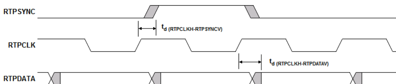
Figure 4-25. RTPDATA Timing
