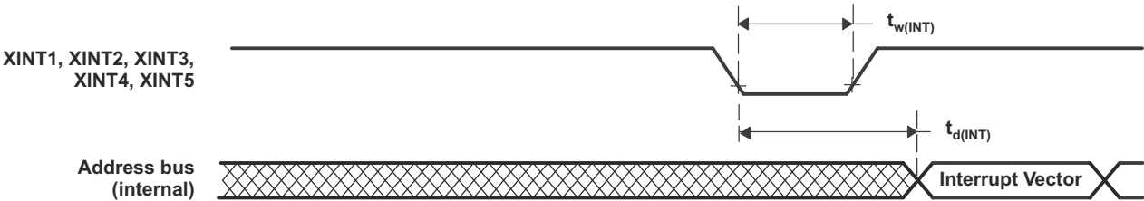
图 7-17. External Interrupt Timing
