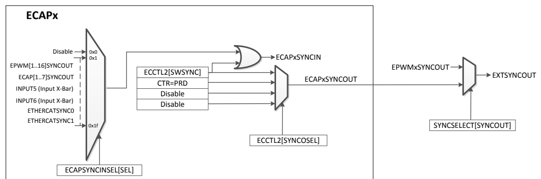
图 7-47. eCAPSynchronization Scheme
