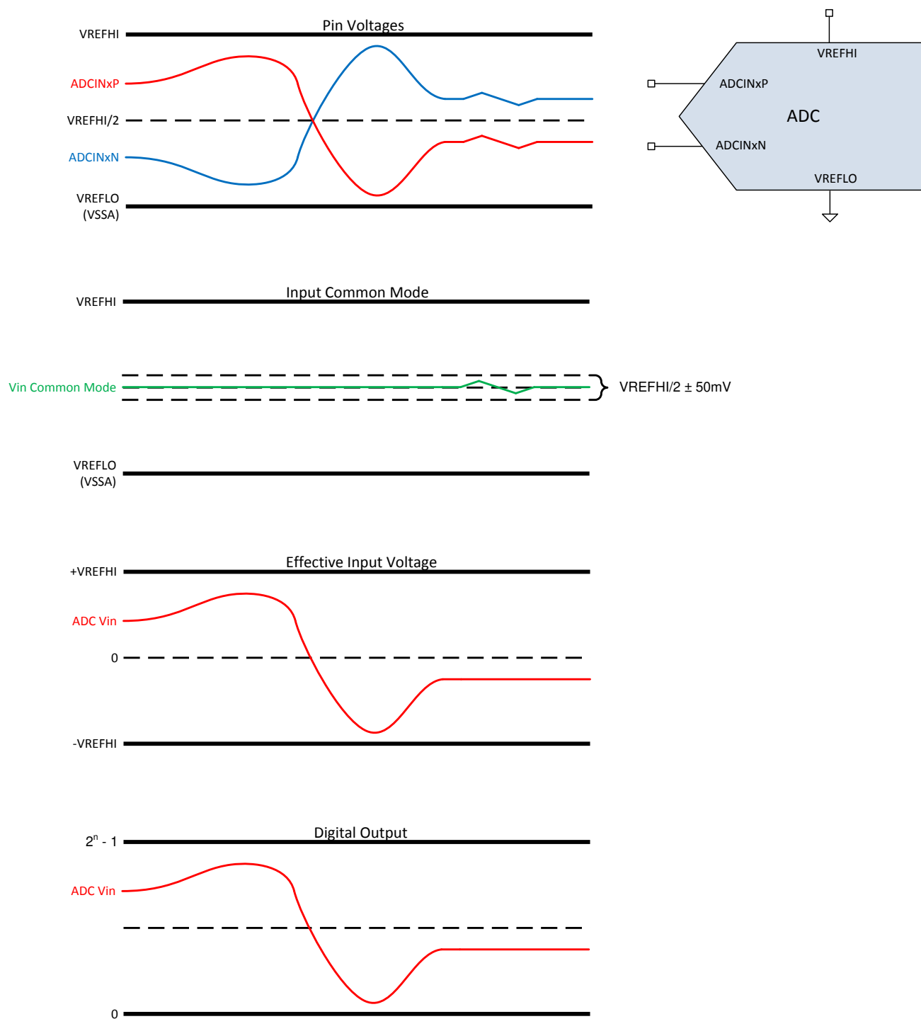
图 7-29. Differential Signaling Mode
