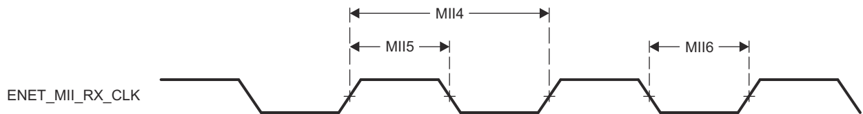
图 7-92. Receive Clock Timing (MII Operation)
