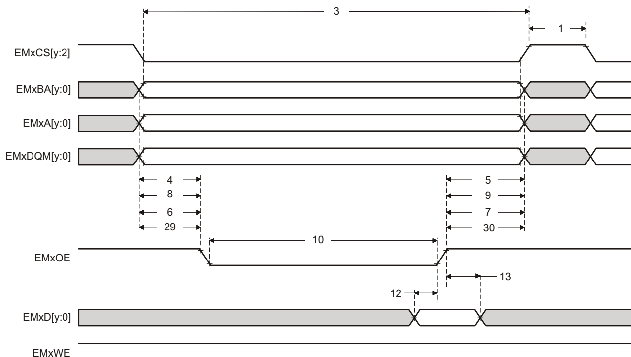
图 7-20. Asynchronous Memory Read Timing
