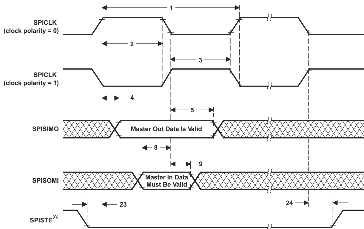
图 7-78. SPI Master Mode External Timing (Clock Phase = 0)
