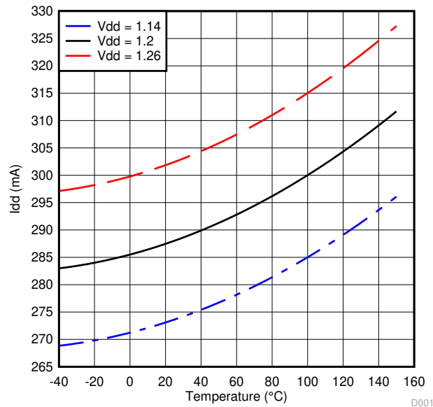
图 7-1. Typical Operating Current Versus Temperature
