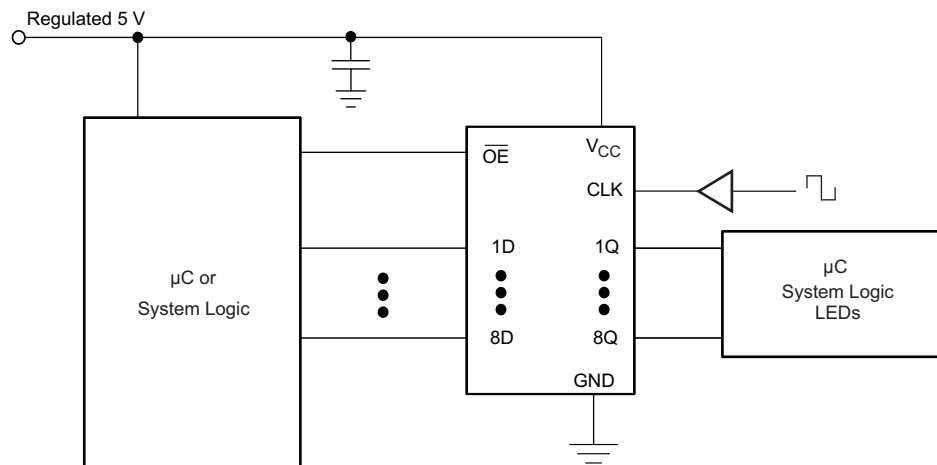
Figure 4. Typical Application Schematic
