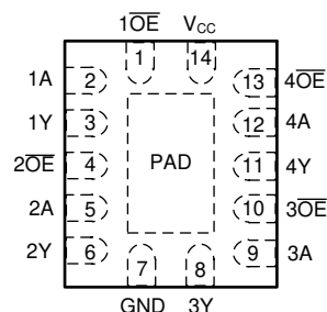
Figure 5-1. BQA Package 14-Pin WQFN Top View
