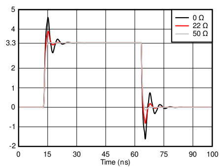
Figure 9-2. Simulated signal integrity at the receiver with different damping resistor ( R_d ) values
