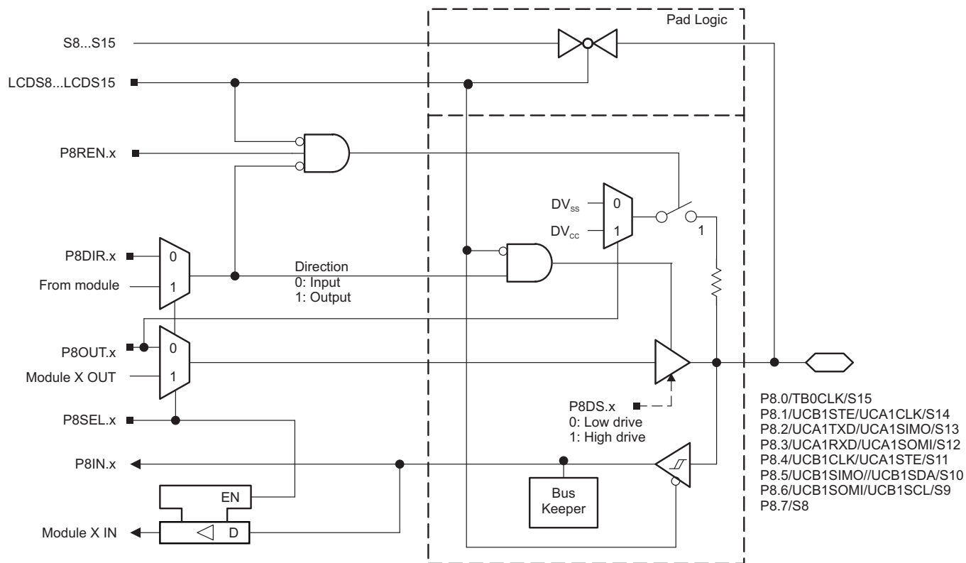
图 6-12. Port P8 (P8.0 to P8.7) Diagram
