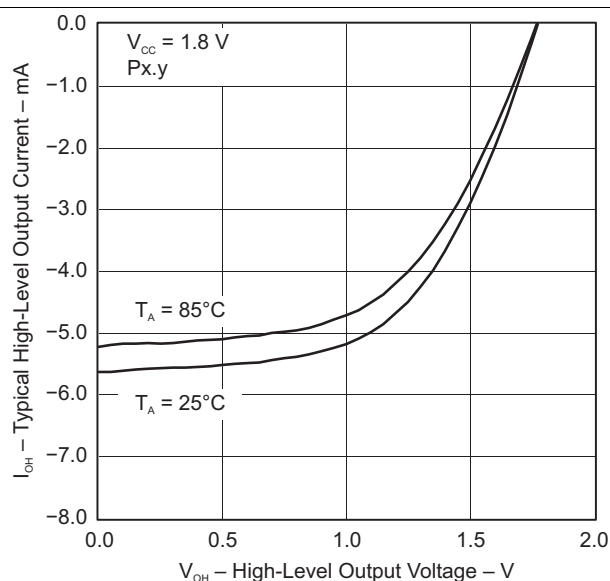
图 5-7. Typical High-Level Output Current vs High-Level Output Voltage
