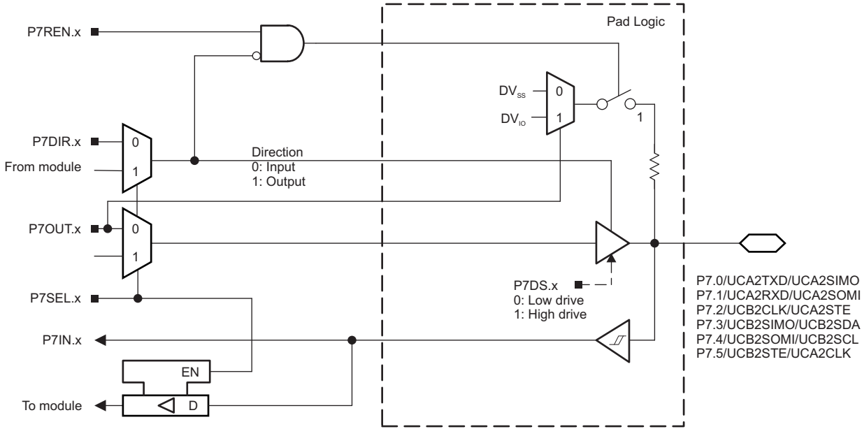
图 6-12. Port P7 (P7.0 to P7.5) Diagram
