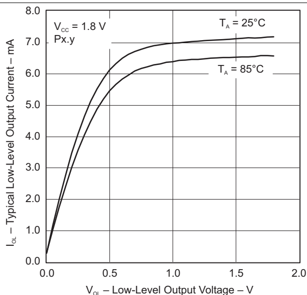
图 5-5. Typical Low-Level Output Current vs Low-Level Output Voltage
