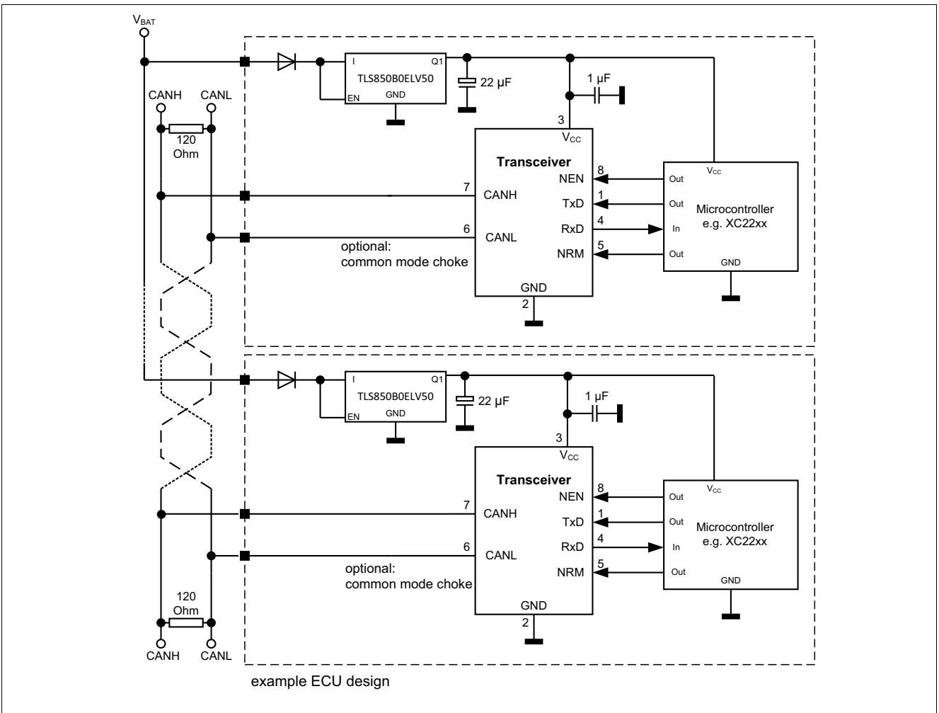
Figure 11 Application circuit
