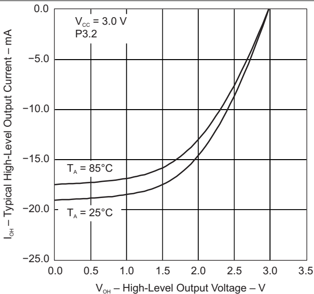
图 5-4. Typical High-Level Output Current vs High-Level Output Voltage
