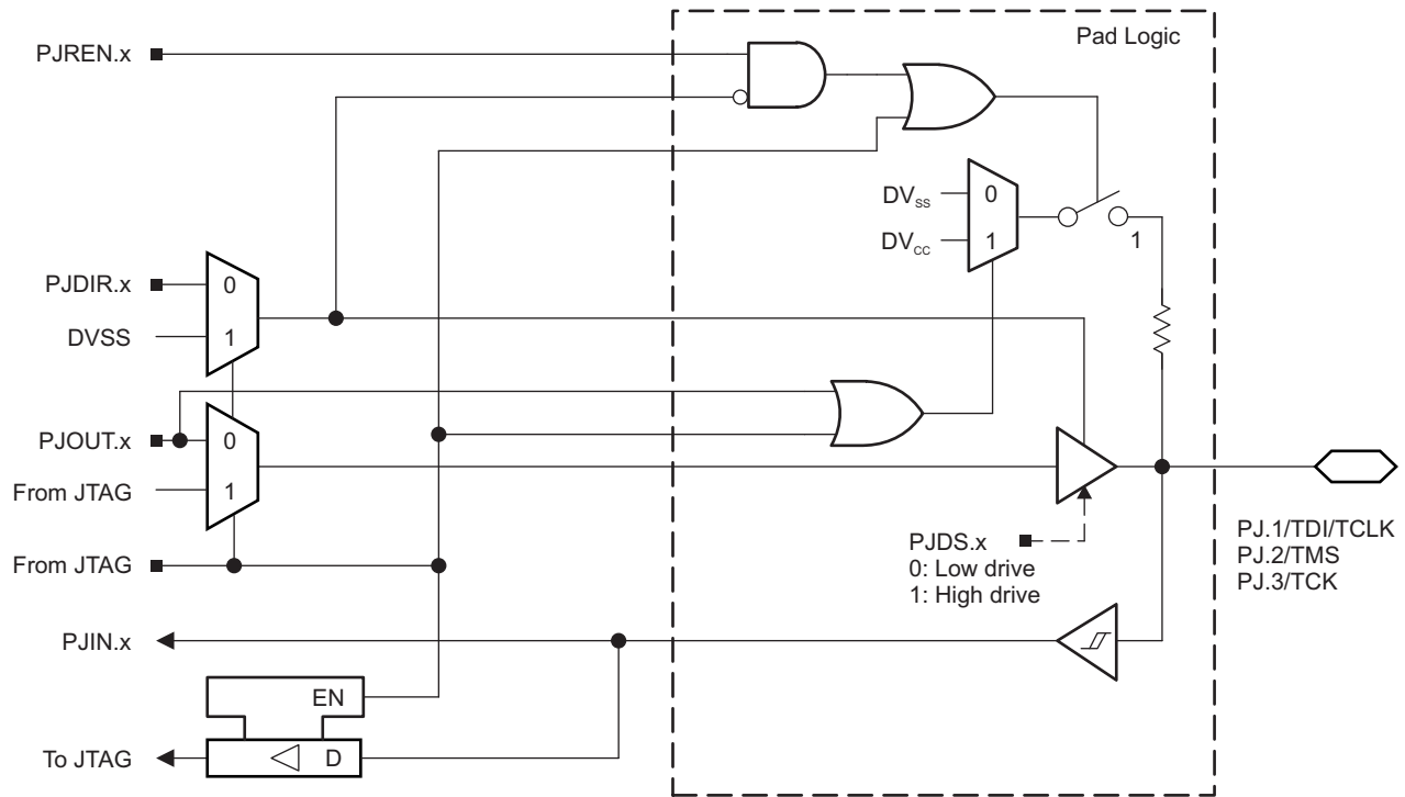
图 6-17. Port PJ (PJ.1 to PJ.3) Diagram
