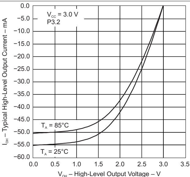
图 5-8. Typical High-Level Output Current vs High-Level Output Voltage
