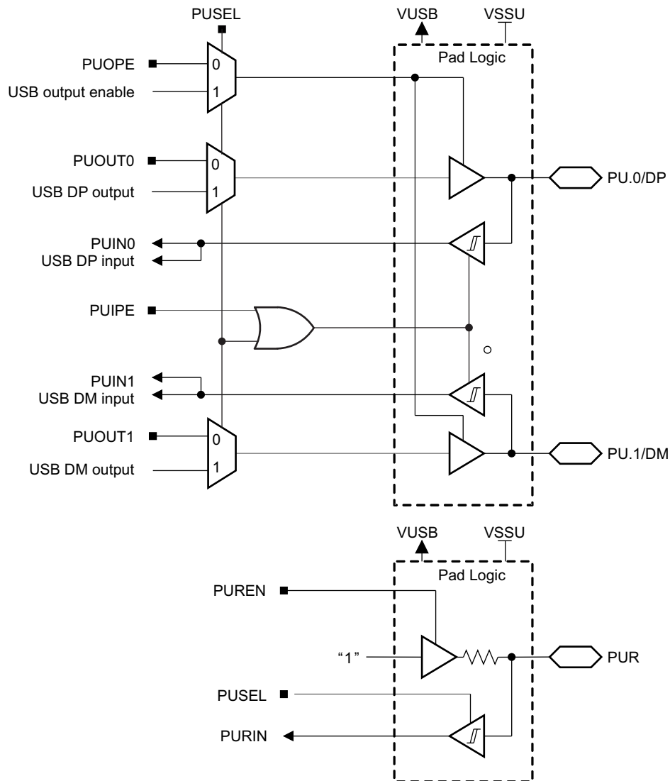
图 6-14. Port PU (PU.0 and PU.1) Diagram (F665x, F565x)
