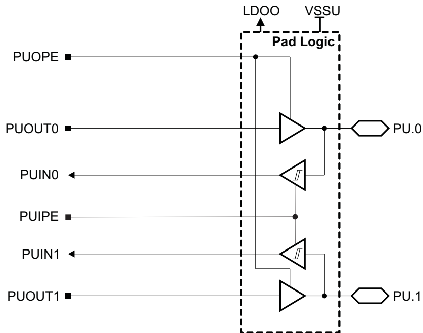
图 6-15. Port PU (PU.0 and PU.1) Diagram (F645x, F535x)
