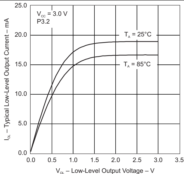
图 5-2. Typical Low-Level Output Current vs Low-Level Output Voltage
