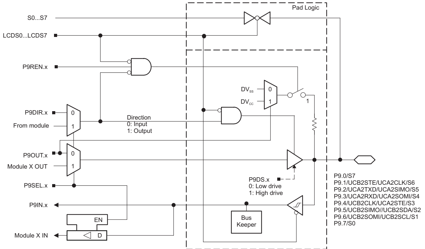
图 6-13. Port P9 (P9.0 to P9.7) Diagram
