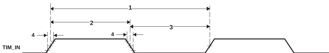
Figure 6-74. Timer Timing
