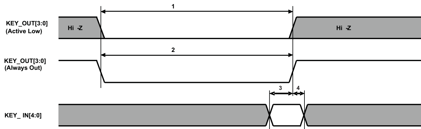
Figure 7-67. Key Scan Timing
