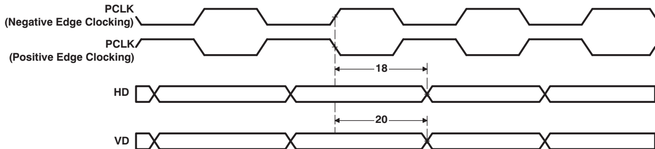
Figure 7-34. VPFE (ISIF) Master Mode Control Output Data Timing
