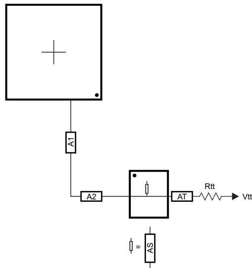
图 7-64. ADDR_CTRL Routing for One DDR3 Device
