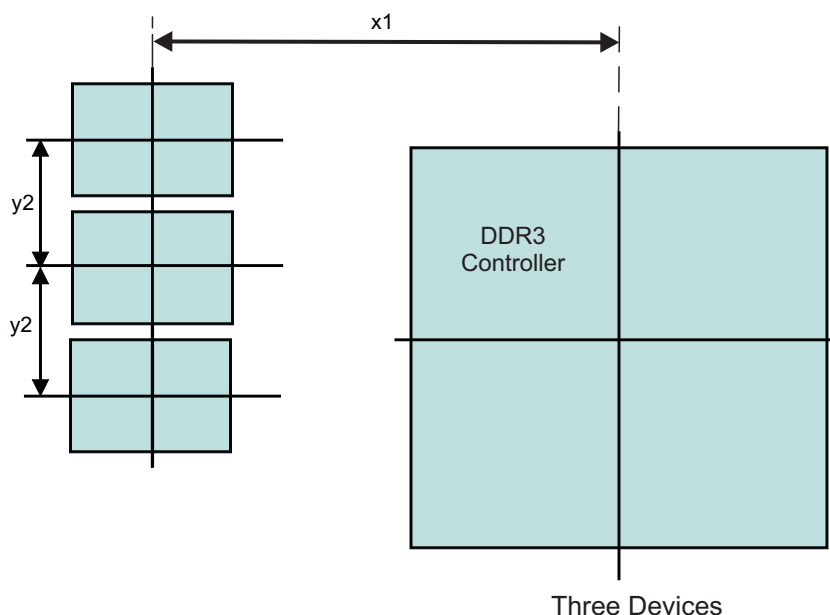
Figure 7-33. Placement Specifications
