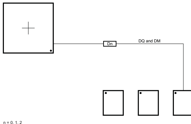
Figure 7-54. DQ/DM Routing With Any Number of Allowed DDR3 Devices
