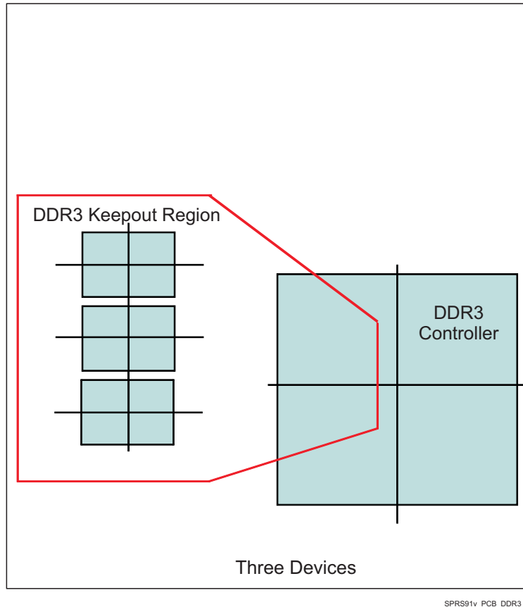
Figure 7-34. DDR3 Keepout Region
