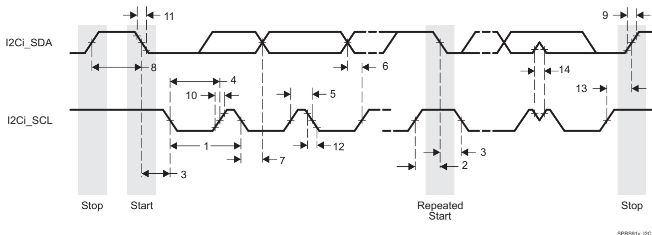
Figure 5-38. I2C Receive Timing
