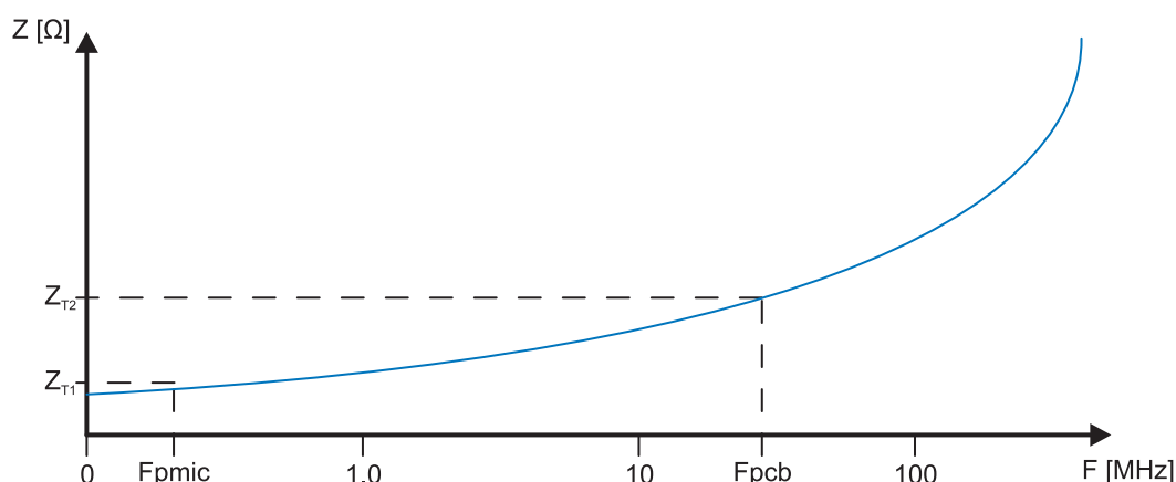
Figure 7-14. PDN's Target impedance
