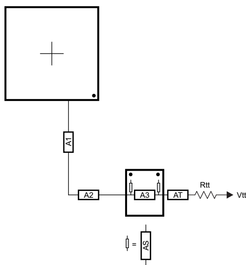
Figure 7-46. ADDR_CTRL Routing for Two Mirrored DDR3 Devices
