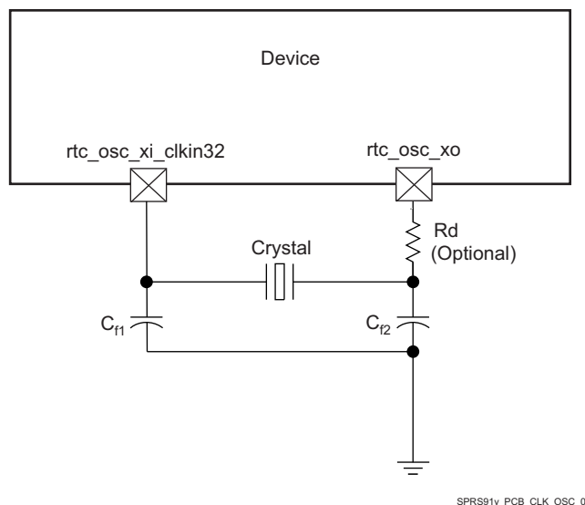
Figure 7-21. Grounding Scheme for Low-Frequency Clock
