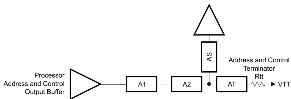
图 7-55. ADDR_CTRL Topology for One DDR3 Device
