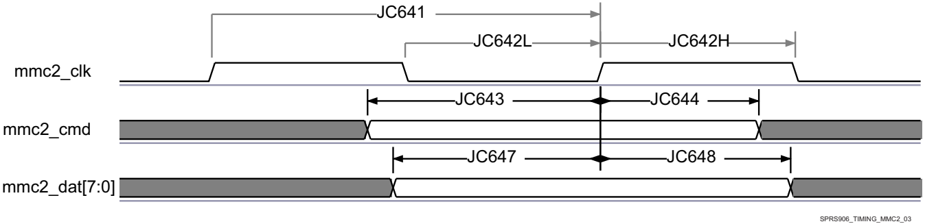
图 5-94. MMC/SD/SDIO in - High Speed JC64 - Receiver Mode
