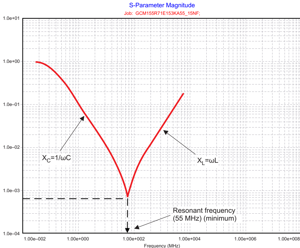
图 7-8. Typical Impedance Profile of a Capacitor
