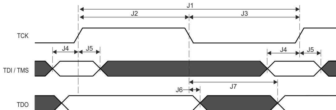
图 8-104. JTAG Test - Port Timing
