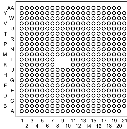
图 7-1. ALM FCBGA-N433 Pin Diagram (Bottom View)
