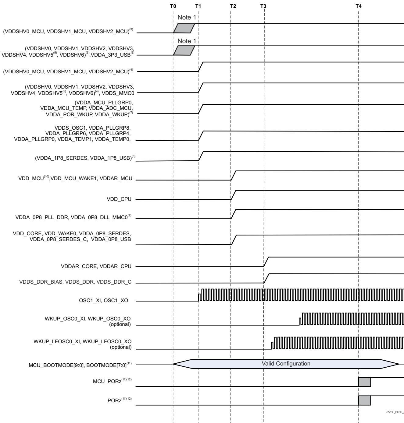
图 8-5. Independent MCU and Main Domains, Primary Power-Up Sequence
