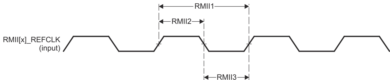
图 8-29. RMII[x]_REFCLK Timing - RMII Mode
