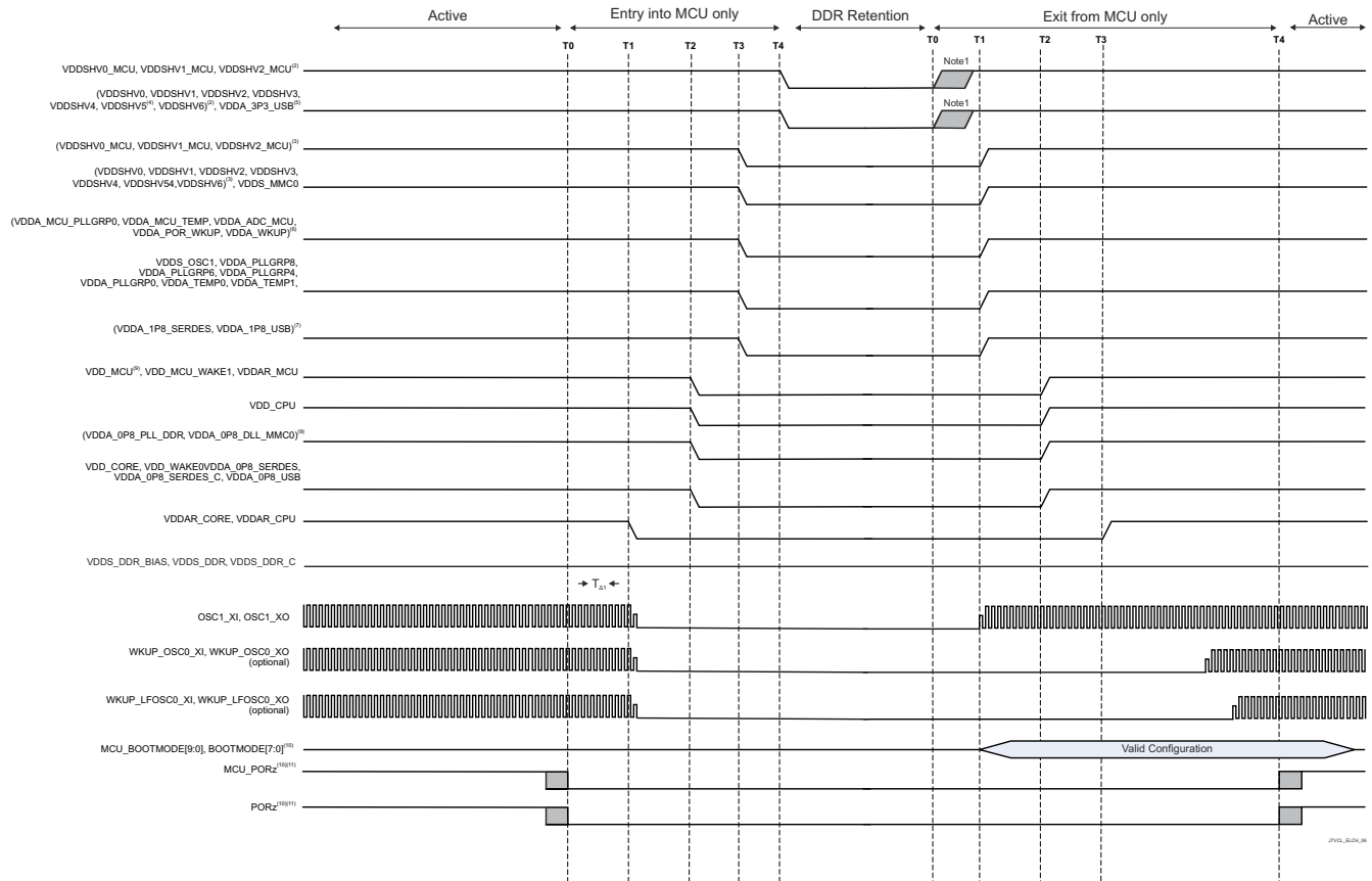
图 8-8. Independent MCU and Main Domains, Entry and Exit of DDR Retention State
