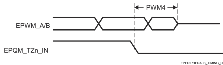
图 8-44. EPWM_A/B and ePWM_TZn_IN Hi - Z Input Timings
