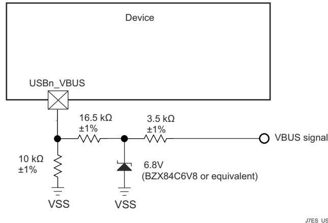
图 10-5. USB VBUS Detect Voltage Divider / Clamp Circuit
