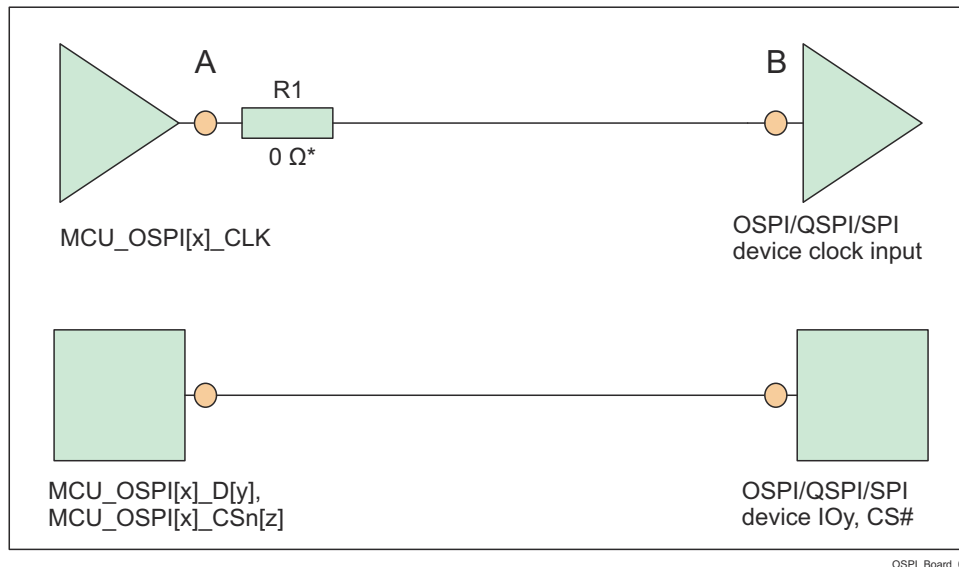
图 10-2. OSPI Interface High Level Schematic
