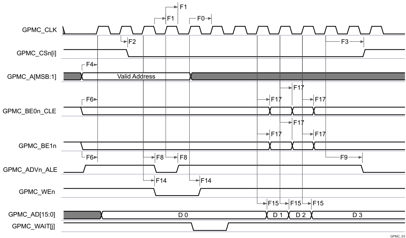
图 8-48. GPMC and NOR Flash — Synchronous Burst Read — 4x16-bit (GPMCFCLKDIVIDER = 0)
