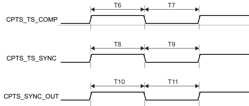
图 8-94. CPTS Output Switching Characteristics
