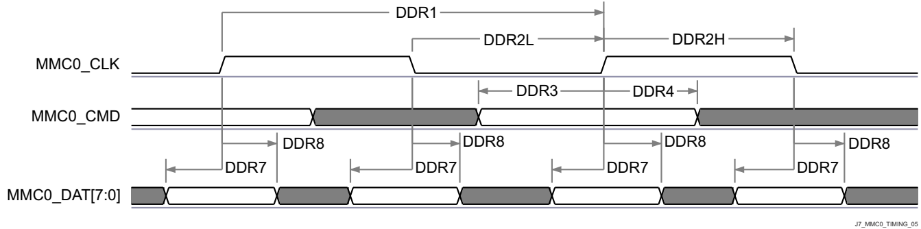
图 8-78. eMMC in - High Speed DDR Mode - Receiver Mode
