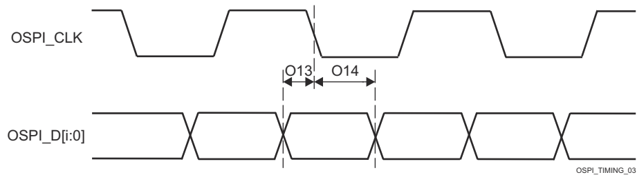
图 8-97. OSPI Timing Requirements - DDR, No Loopback Clock and Internal Pad Loopback Clock
