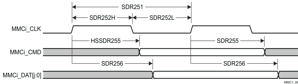
图 8-89. SD/SDIO in – High Speed SDR25 – Transmitter Mode
