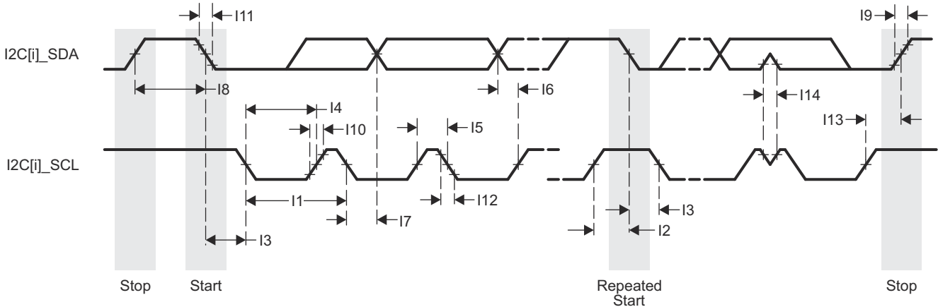
图 8-65. I2C Receive Timing
