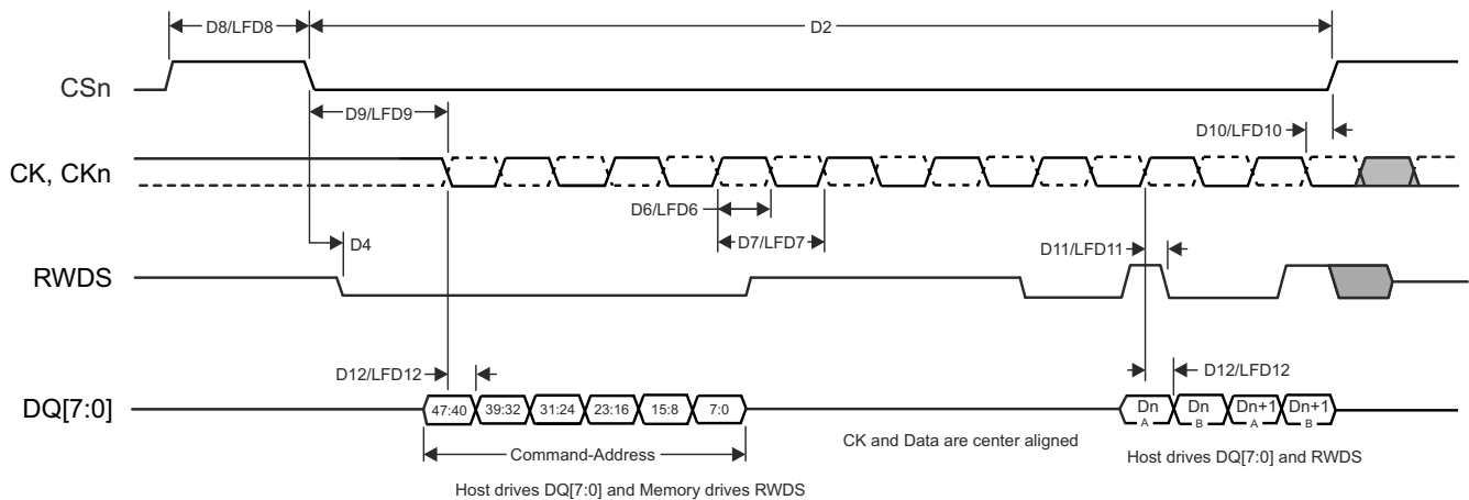
图 8-62. HyperBus Timing Diagrams – Transmitter Mode
