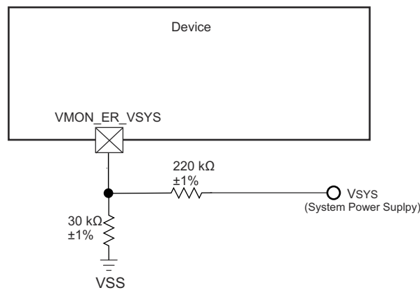
图 10-6. System Supply Monitor Voltage Divider Circuit
