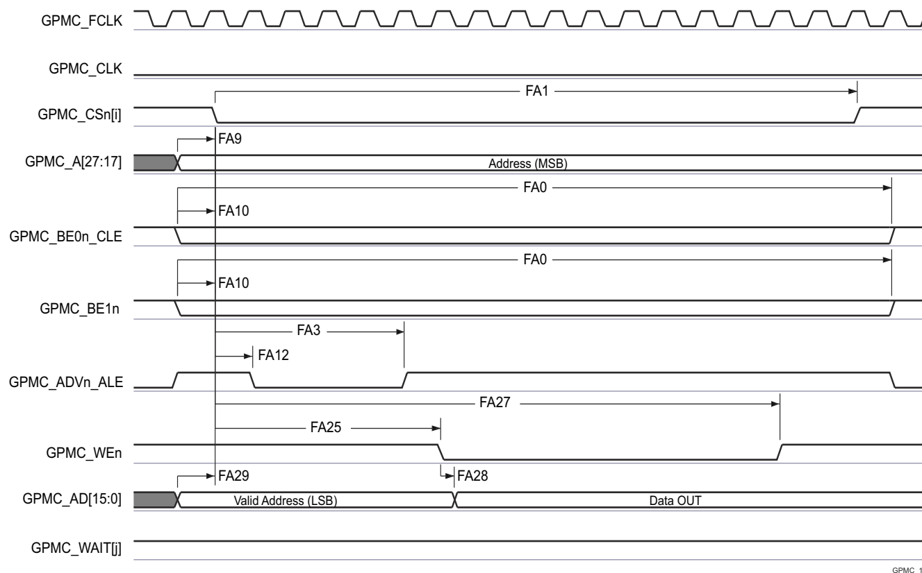
图 8-57. GPMC and Multiplexed NOR Flash — Asynchronous Write — Single Word
