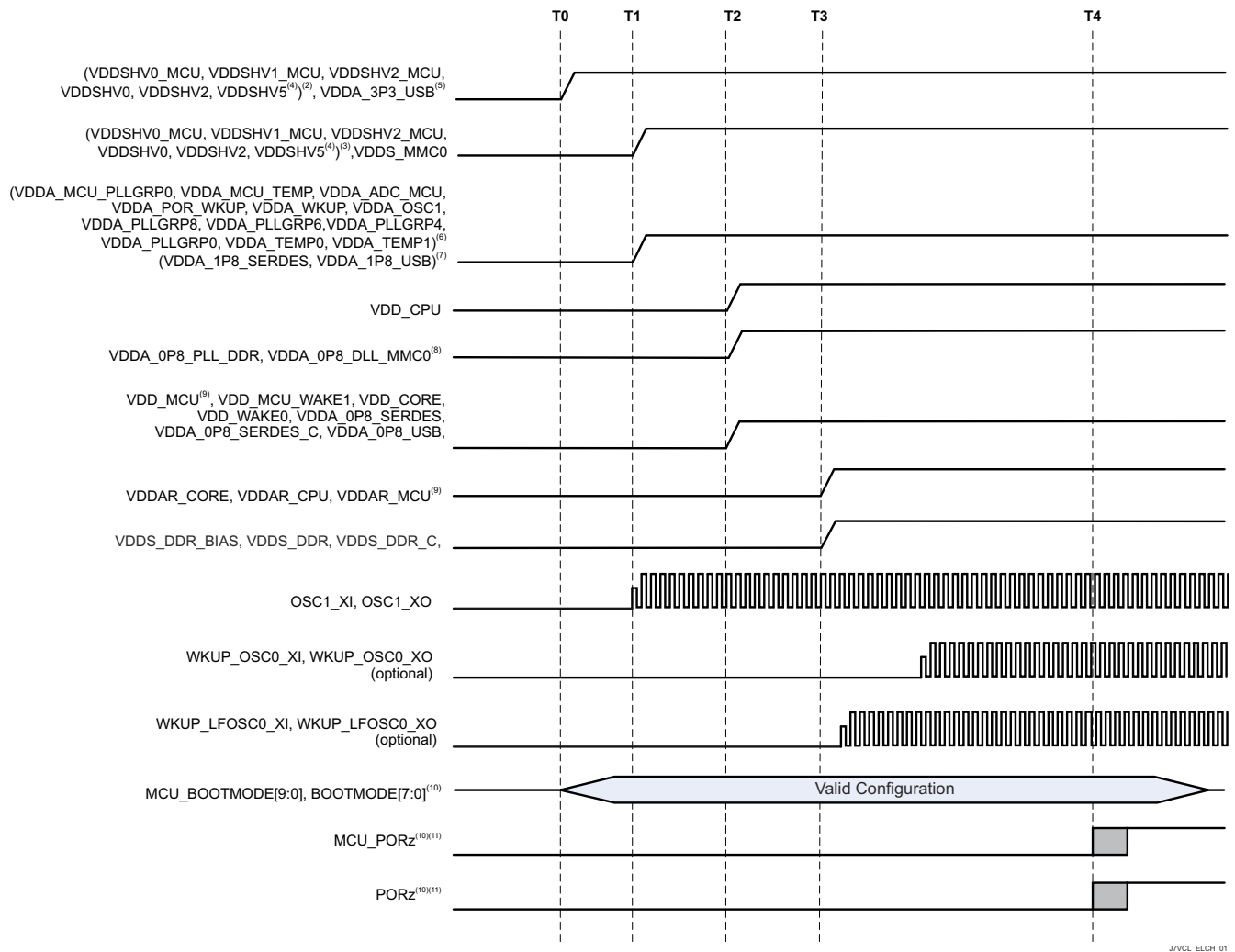
图 8-3. Combined MCU and Main Domains, Primary Power-Up Sequence
