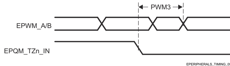
图 8-43. EPWM_A/B and ePWM_TZn_IN Forced High/Low Input Timings
