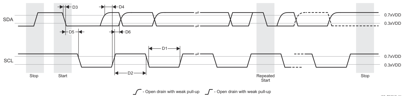
图 8-66. I3C Open Drain Timing
