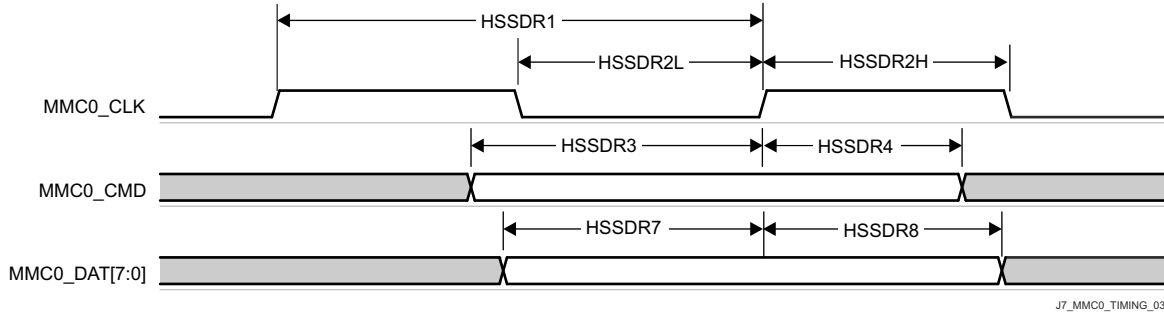
图 8-76. eMMC in - High Speed SDR Mode - Receiver Mode
