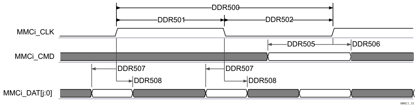
图 8-91. SD/SDIO - High Speed SD - DDR - Data/Command Receive
