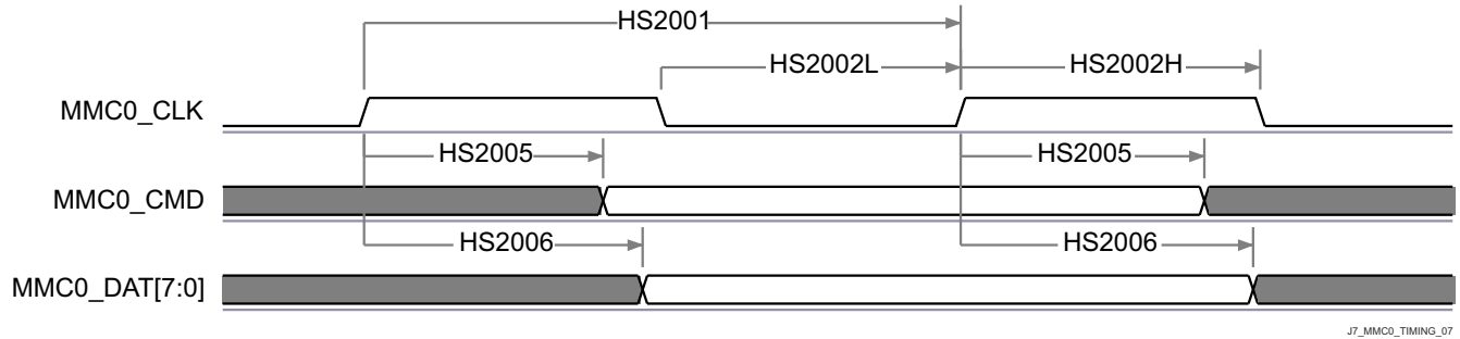
图 8-80. eMMC in - HS200 Mode - Transmitter Mode
