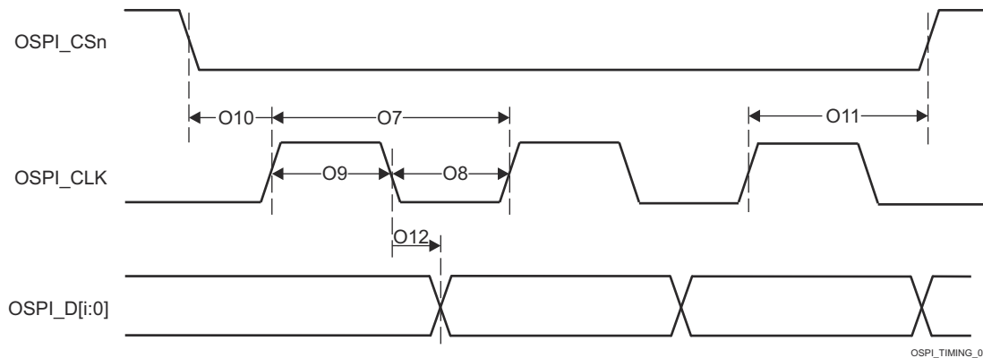
图 8-96. OSPI Switching Characteristics - SDR
