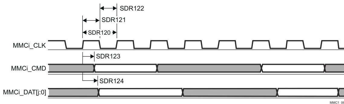
图 8-87. SD/SDIO in - High Speed SDR12 - Transmitter Mode
