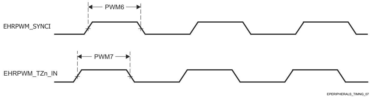
图 8-45. ePWM_SYNCI and ePWM_TZn_IN Output Timings
