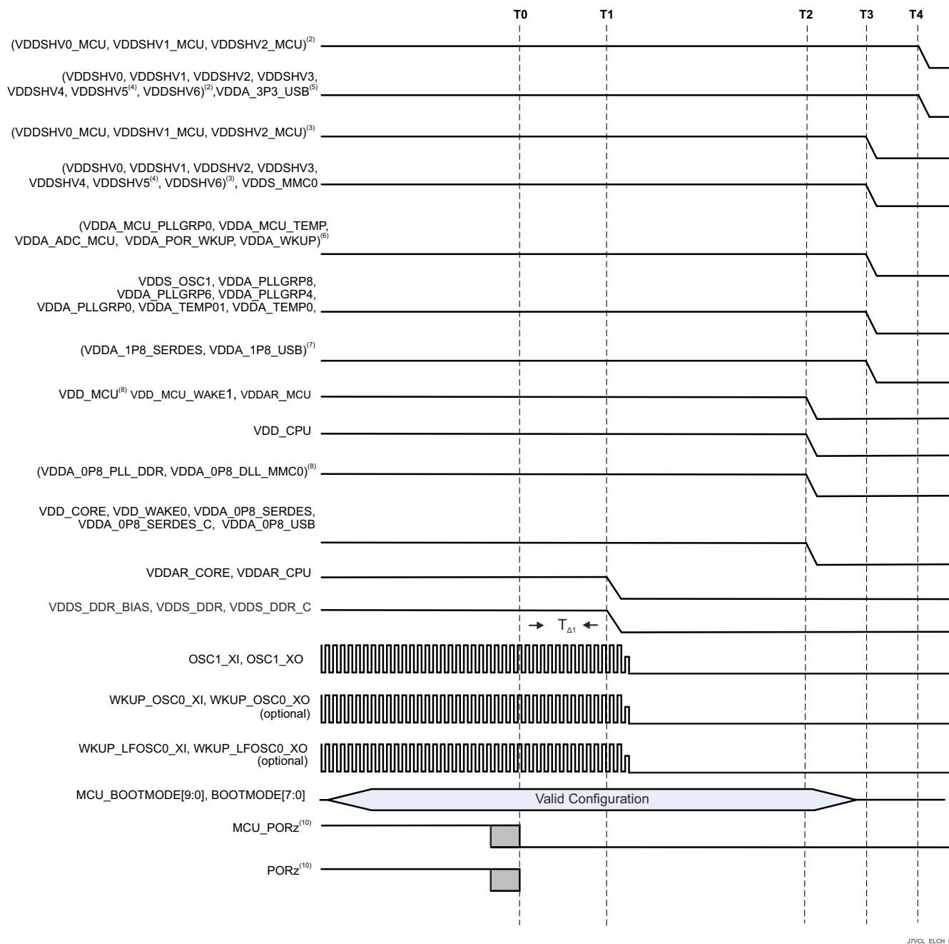
图 8-6. Independent MCU and Main Domains, Primary Power- Down Sequencing
