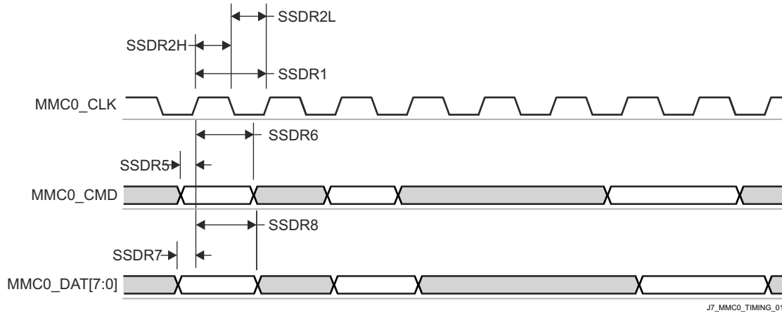
图 8-74. eMMC in - Default Speed - Receiver Mode
