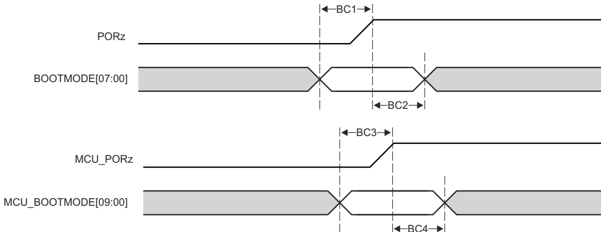
图 8-12. Boot Configuration Timing
