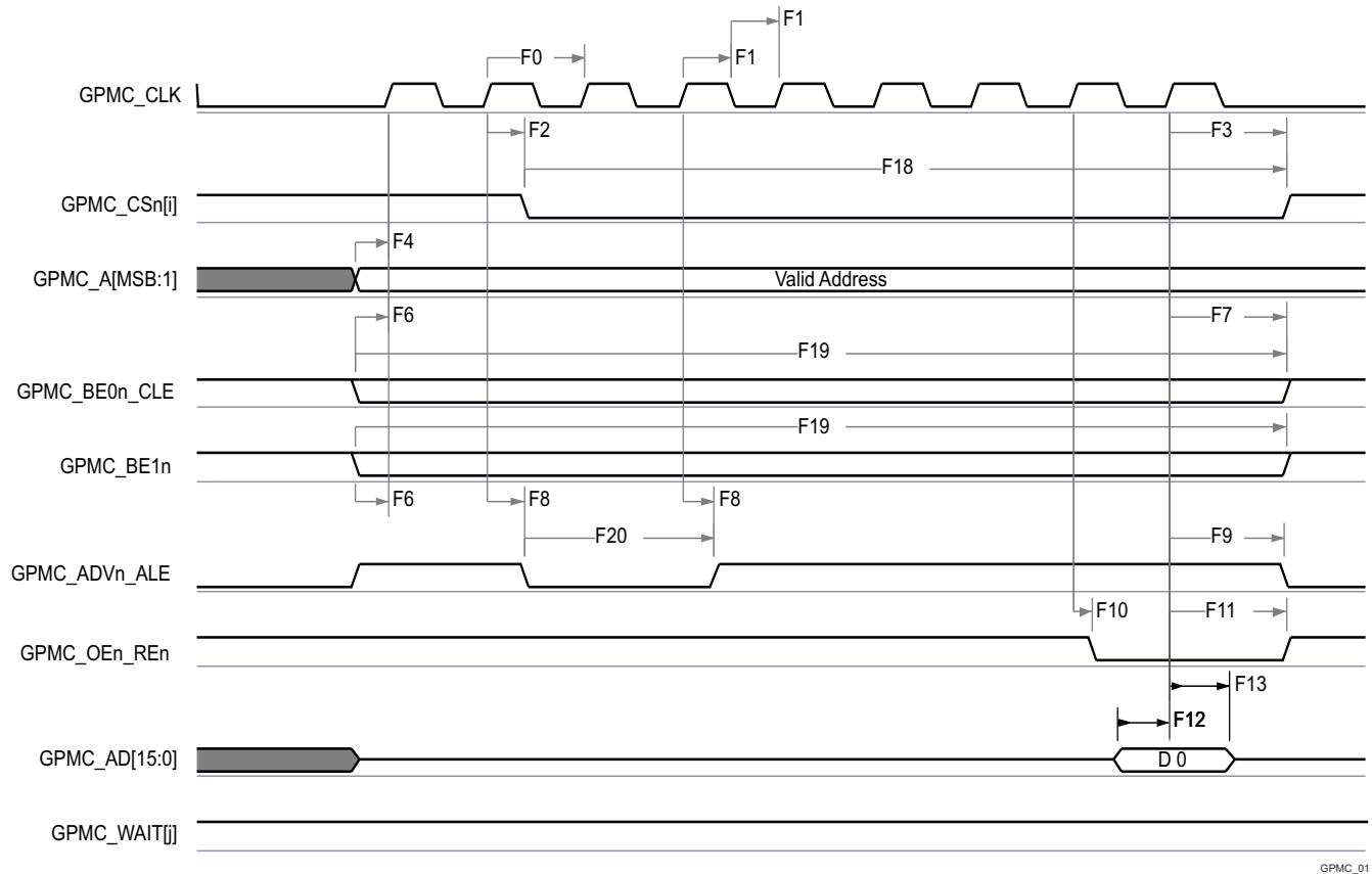
图 8-47. GPMC and NOR Flash — Synchronous Single Read (GPMCFCLKDIVIDER = 0)
