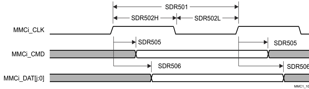
图 8-90. SD/SDIO in - High Speed SDR50 - Transmitter Mode
