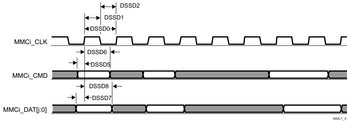
图 8-82. SD/SDIO in - Default Speed - Receiver Mode
