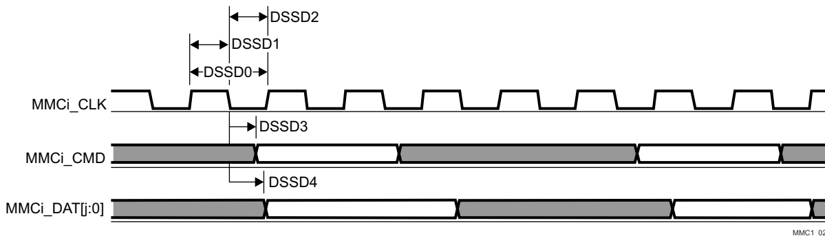
图 8-83. SD/SDIO in - Default Speed - Transmitter Mode
