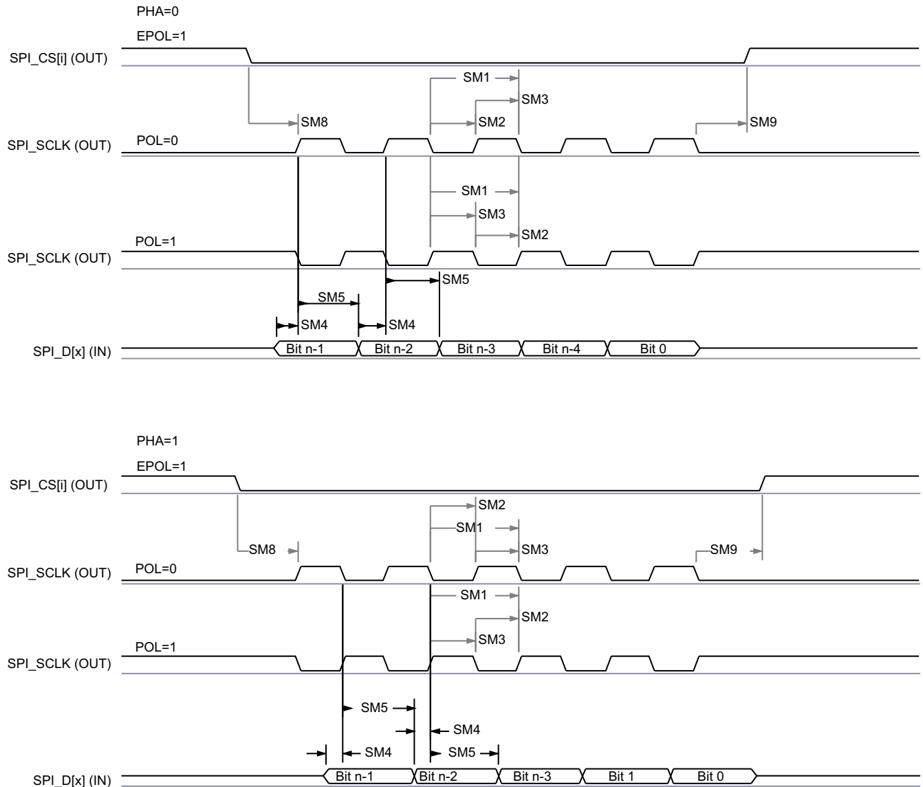
图 8-70. SPI Master Mode Receive Timing
