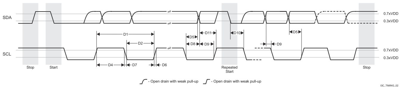
图 8-67. I3C Push-Pull Timing (SDR and HDR-DDR Modes)
