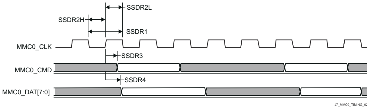
图 8-75. eMMC in - Default Speed - Transmitter Mode
