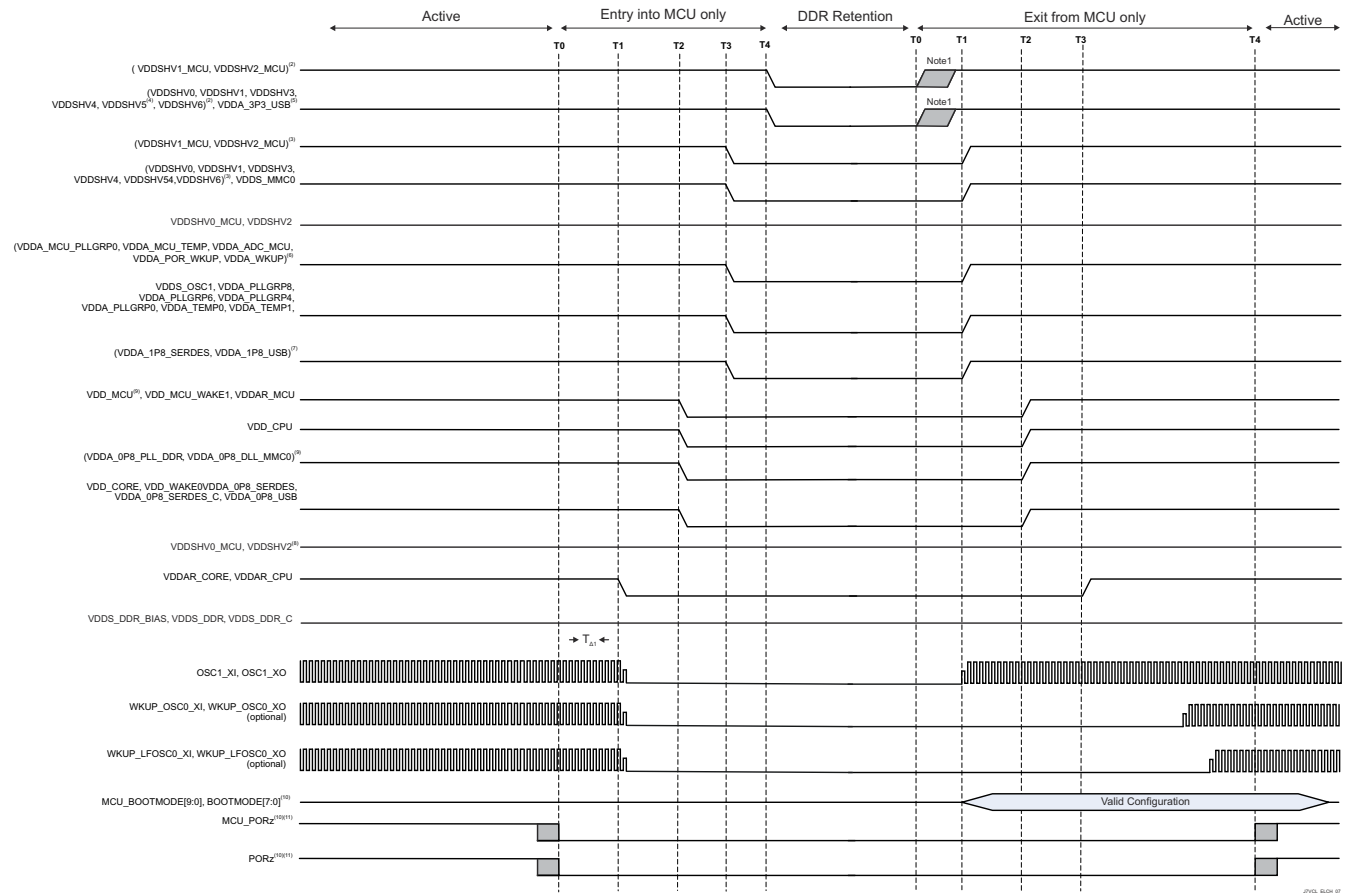
图 8-9. Independent MCU and Main Domains, Entry and Exit of GPIO Retention Sequencing
