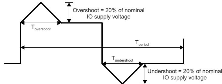
图 8-1. IO Transient Voltage Ranges
