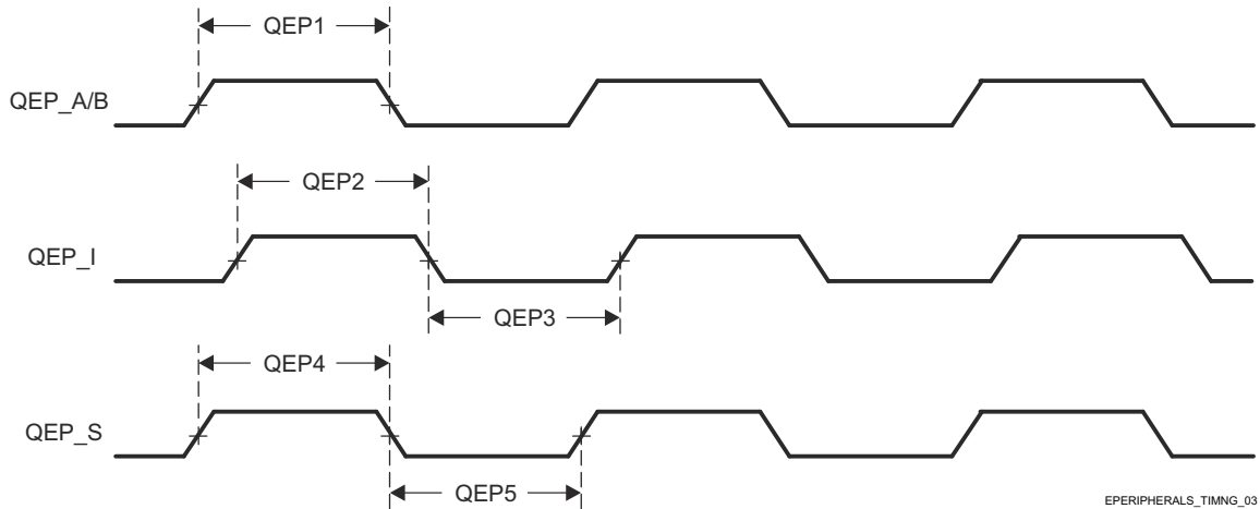
图 8-46. EQEP Input Timings
