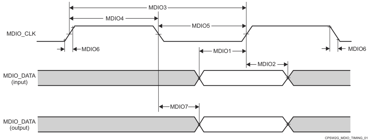
图 8-34. CPSW5G MDIO Diagrams Receive and Transmit
