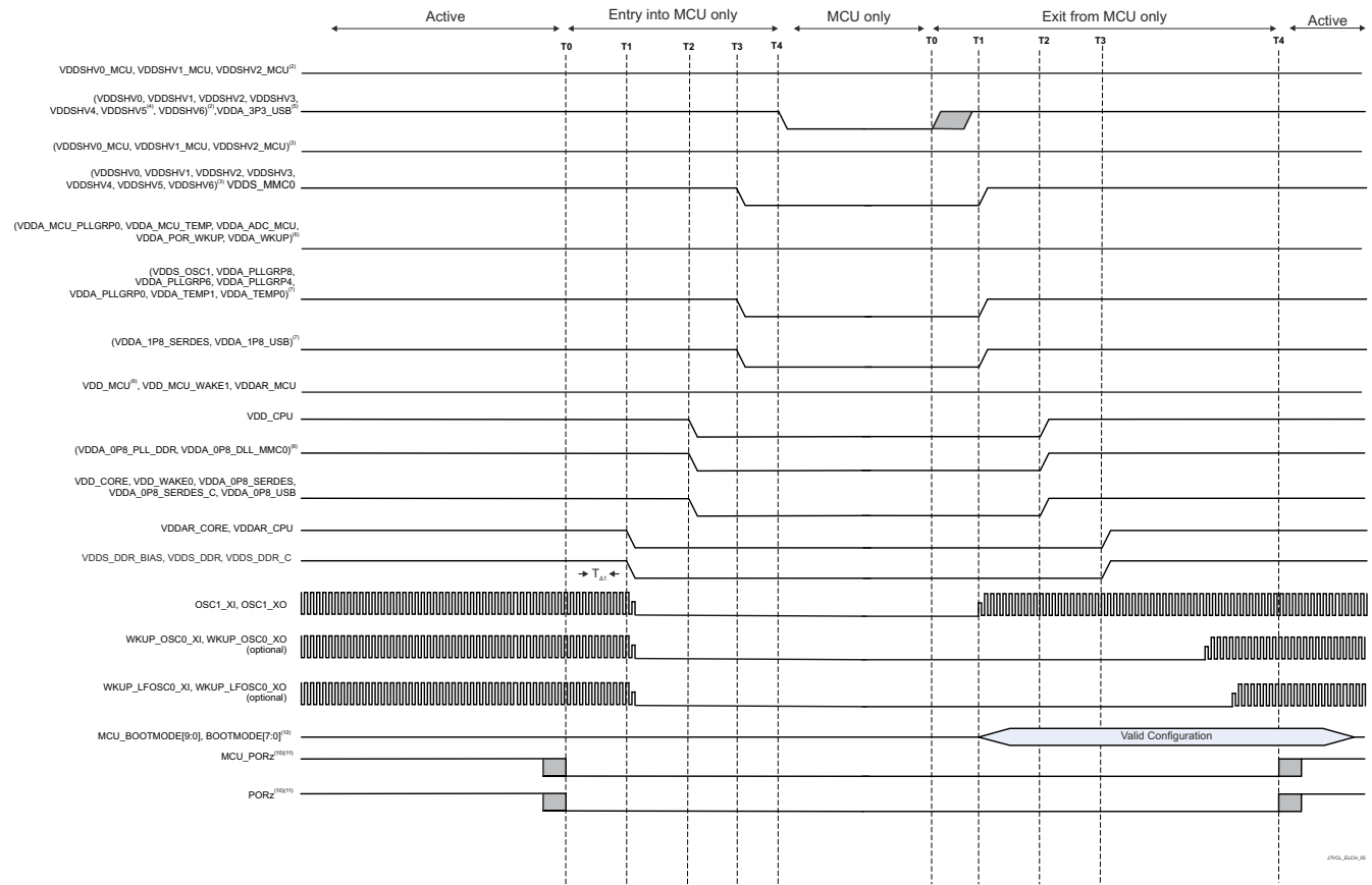
图 8-7. Independent MCU and Main Domains, Entry and Exit of MCU Only Sequencing
