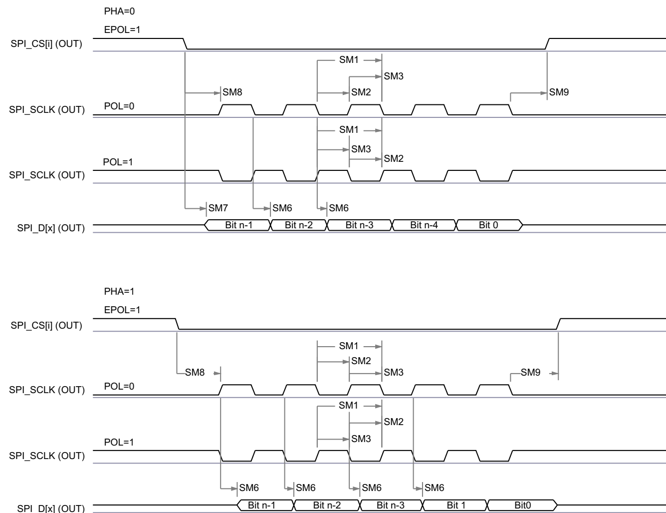
图 8-71. SPI Master Mode Transmit Timing
