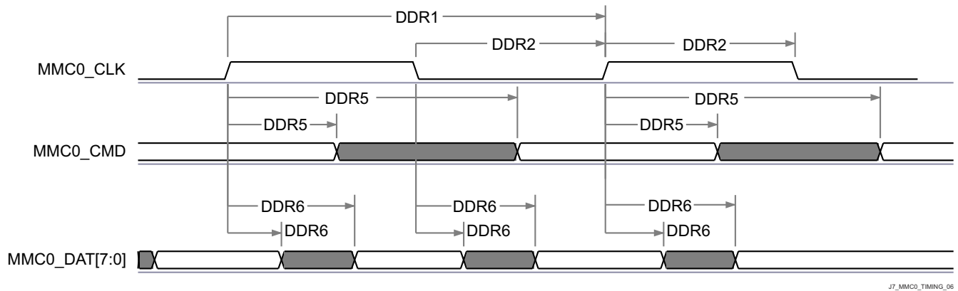
图 8-79. eMMC in - High Speed DDR Mode - Transmitter Mode
