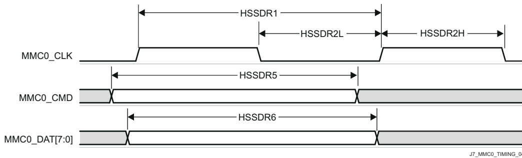
图 8-77. eMMC in - High Speed SDR Mode - Transmitter Mode
