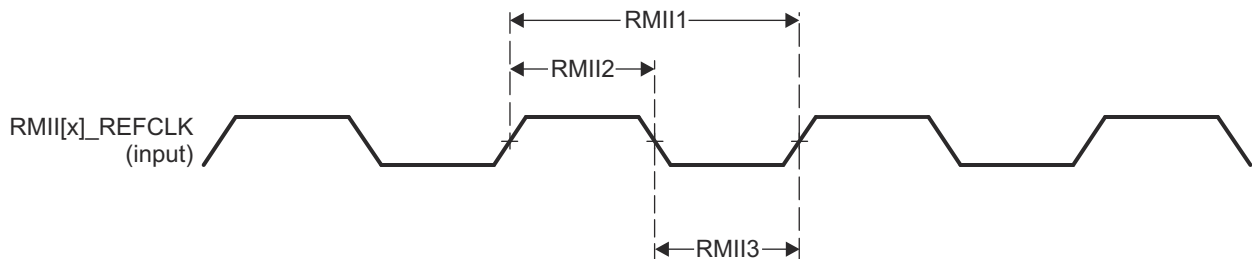
图 8-35. RMII[x]_REFCLK Timing - RMII Mode
