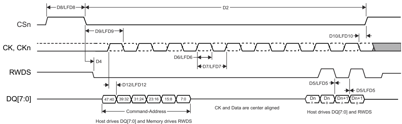
图 8-63. HyperBus Timing Diagrams – Receiver Mode
