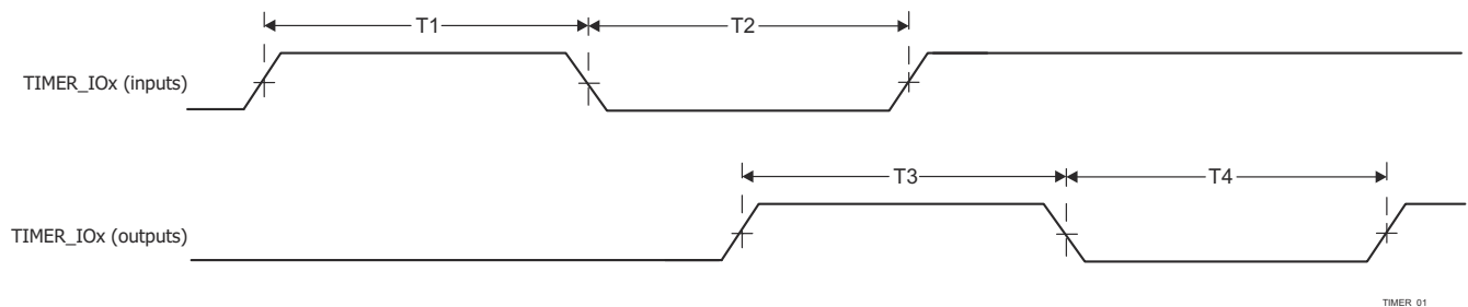
图 8-101. Timer Timing
