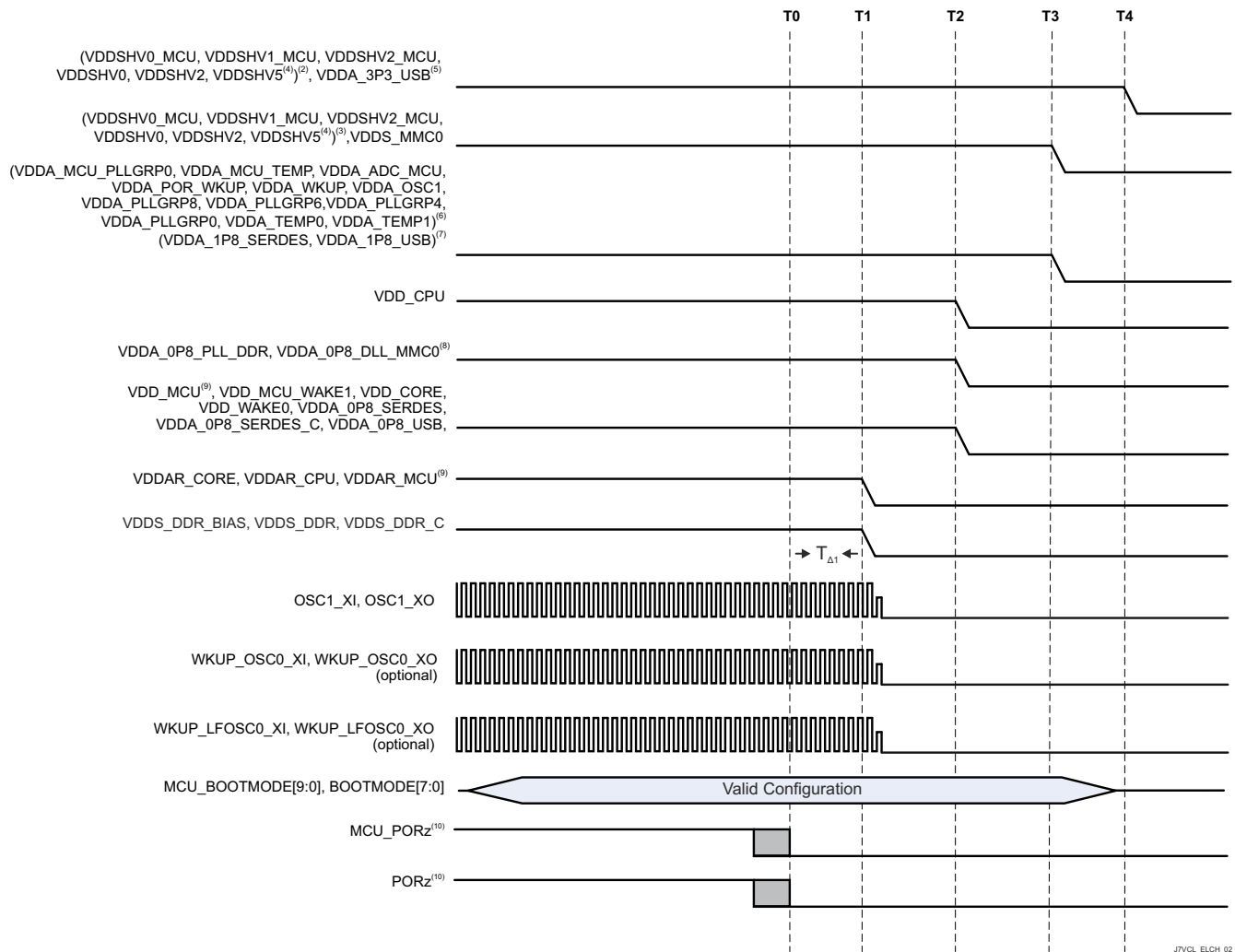
图 8-4. Combined MCU and Main Domains, Primary Power-Down Sequence
