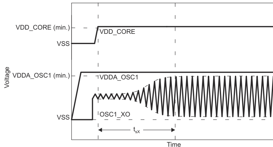
图 8-20. OSC1 Start-up Time
