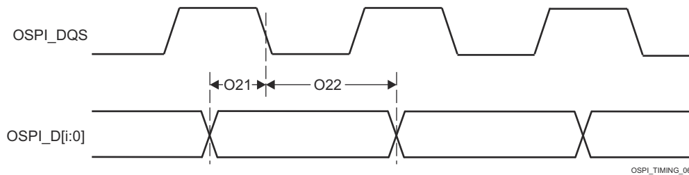
图 8-100. OSPI Timing Requirements - SDR, External Loopback Clock
