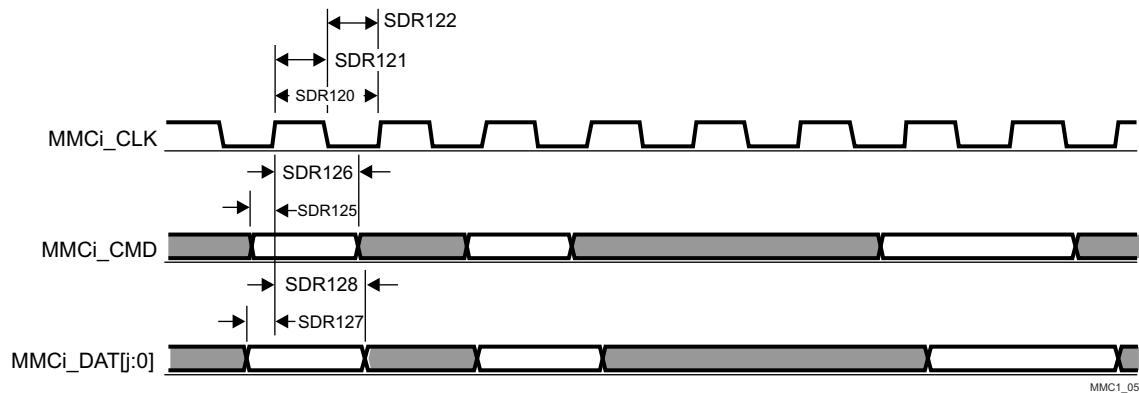
图 8-86. SD/SDIO in - High Speed SDR12 - Receiver Mode
