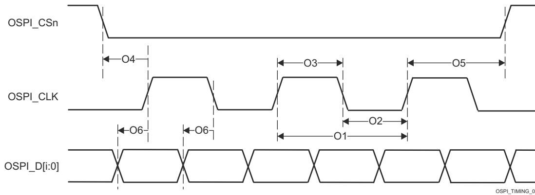
图 8-95. OSPI Switching Characteristics - DDR
