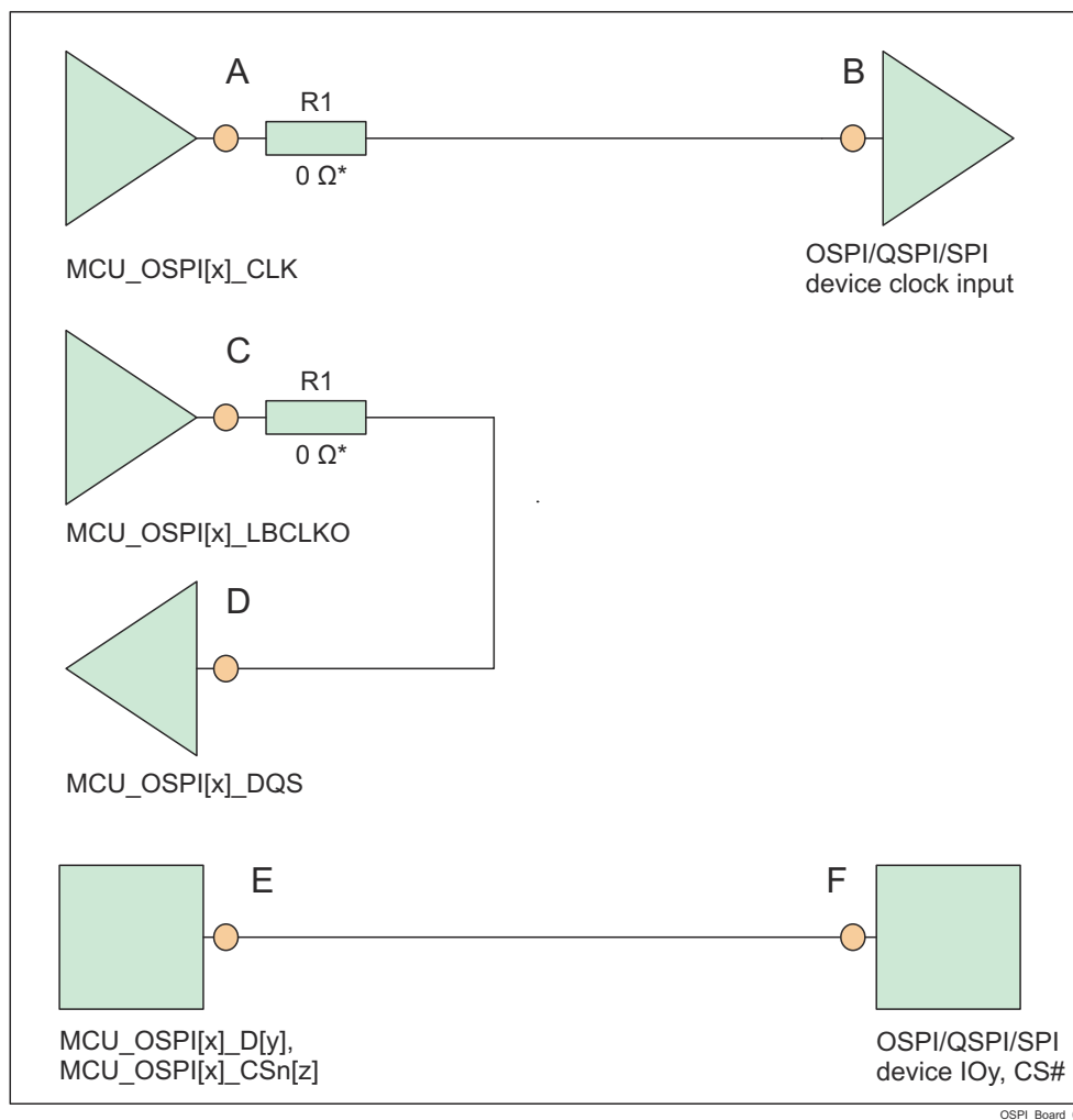
图 10-3. OSPI Interface High Level Schematic
