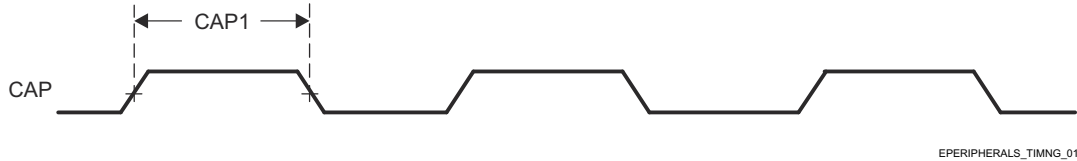
图 8-40. ECAP Input Timings
