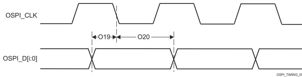
图 8-99. OSPI Timing Requirements - SDR, No Loopback Clock and Internal Pad Loopback Clock
