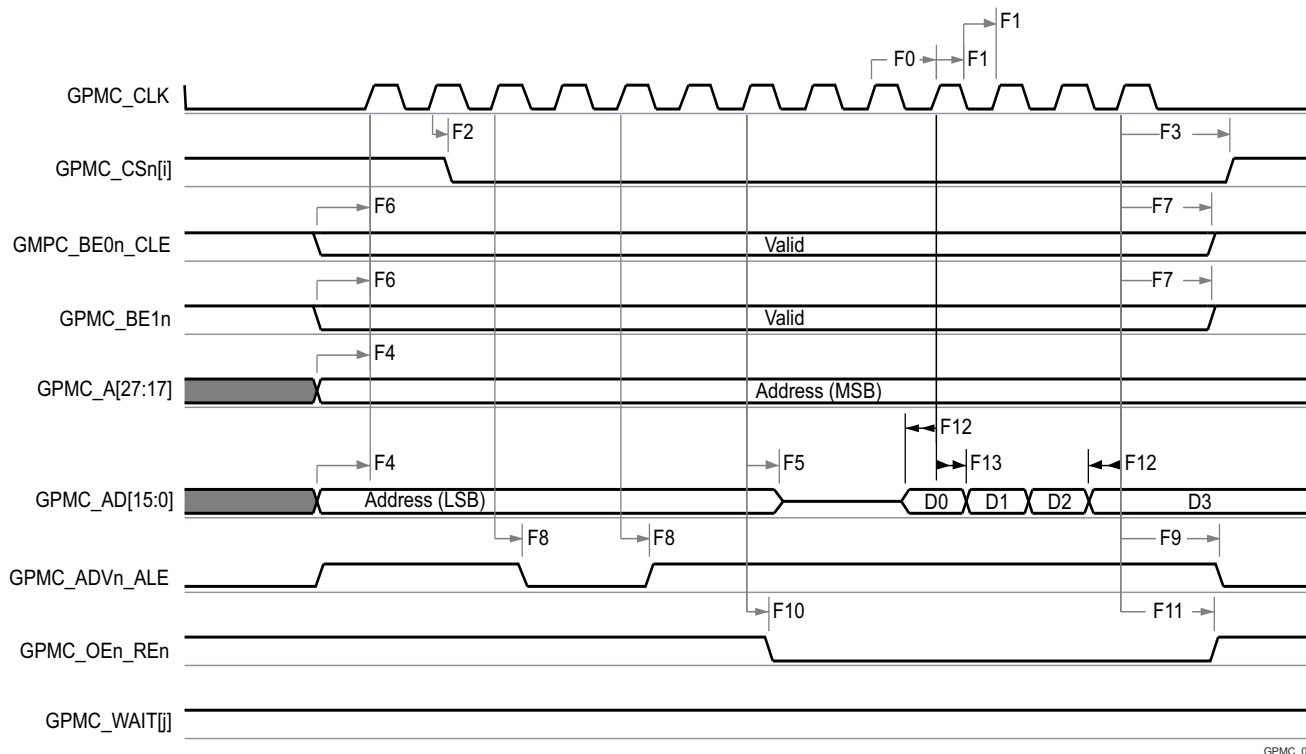
图 8-49. GPMC and NOR Flash—Synchronous Burst Write (GPMCFCLKDIVIDER = 0)
