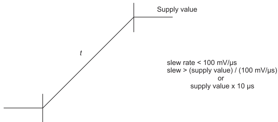
图 8-2. Power Supply Slew and Slew Rate
