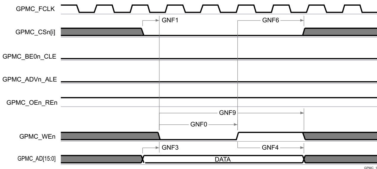
图 8-60. GPMC and NAND Flash — Data Read Cycle
