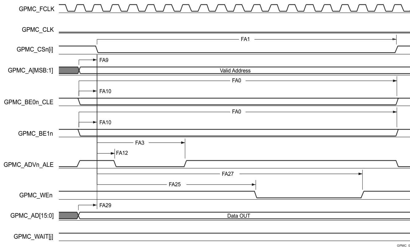
图 8-55. GPMC and NOR Flash — Asynchronous Write — Single Word
