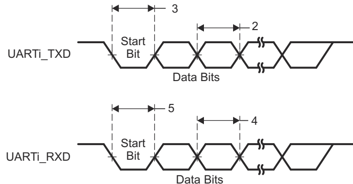
图 8-102. UART Timing
