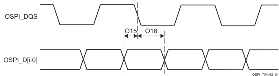
图 8-98. OSPI Timing Requirements - DDR, External Loopback Clock and DQS
