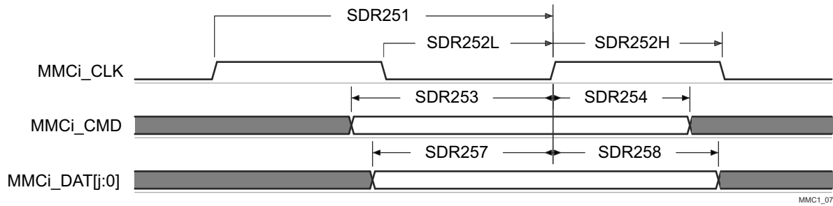
图 8-88. SD/SDIO in – High Speed SDR25 – Receiver Mode
