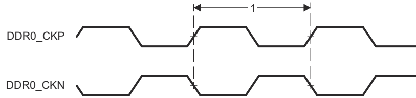
图 8-39. DDRSS Memory Interface Clock Timing
