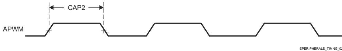
图 8-41. ECAP Output Timings
