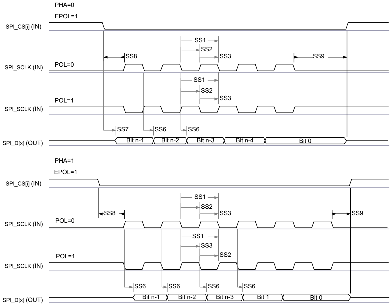
图 8-73. SPI Slave Mode Transmit Timing
