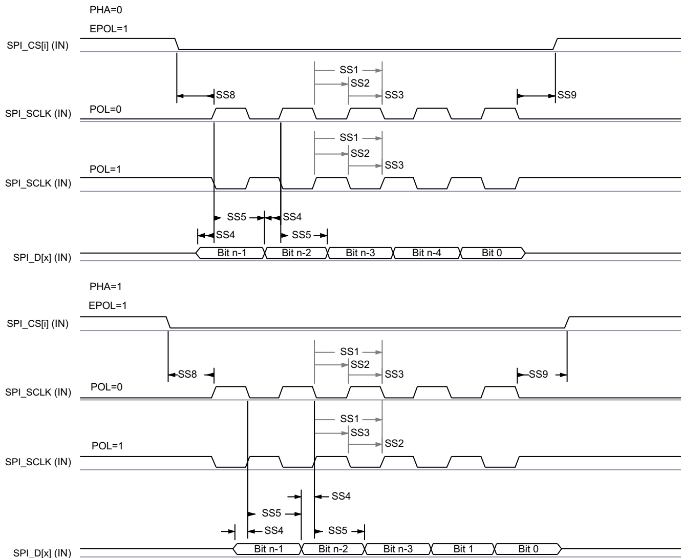
图 8-72. SPI Slave Mode Receive Timing
