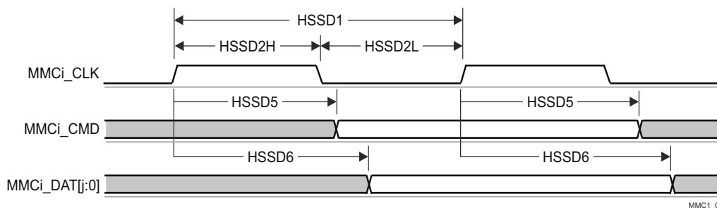
图 8-85. SD/SDIO in – High Speed – Transmitter Mode
