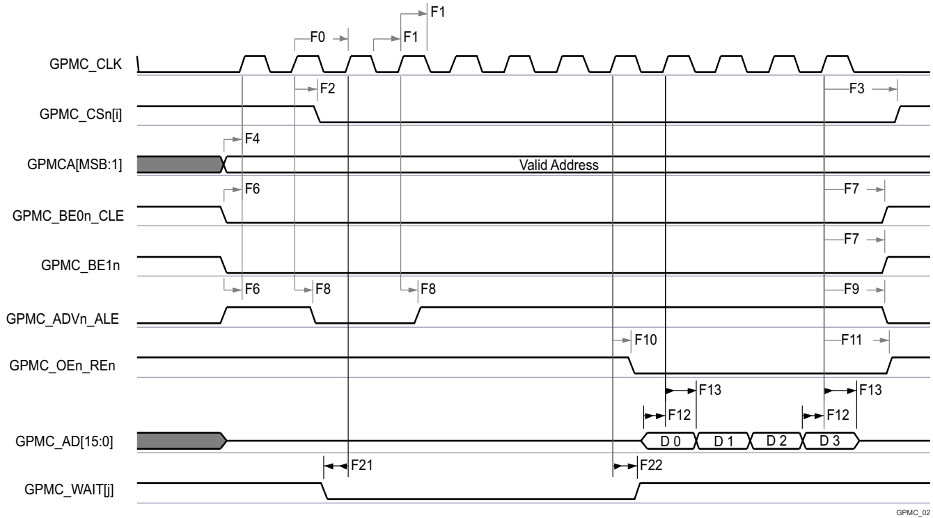
图 8-48. GPMC and NOR Flash — Synchronous Burst Read — 4x16-bit (GPMCFCLKDIVIDER = 0)
