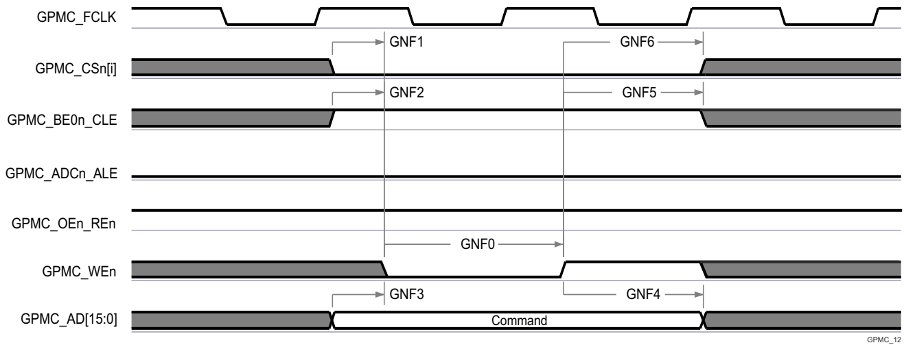
图 8-58. GPMC and NAND Flash — Command Latch Cycle
