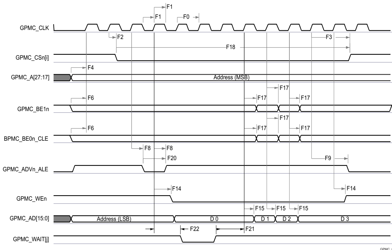
图 8-51. GPMC and Multiplexed NOR Flash — Synchronous Burst Write
