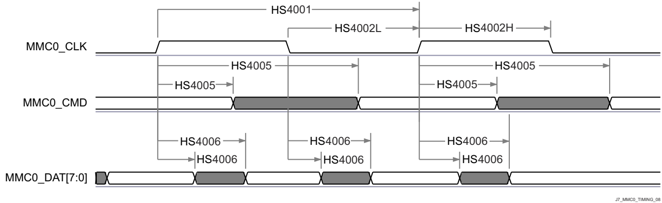
图 8-81. eMMC in - HS400 Mode - Transmitter Mode
