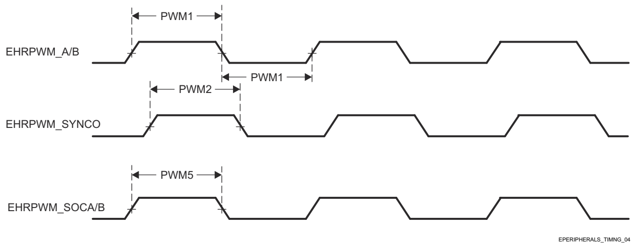
图 8-42. EPWM_A/B_out, ePWM_SYNCO, and ePWM_SOCA/B Input Timings
