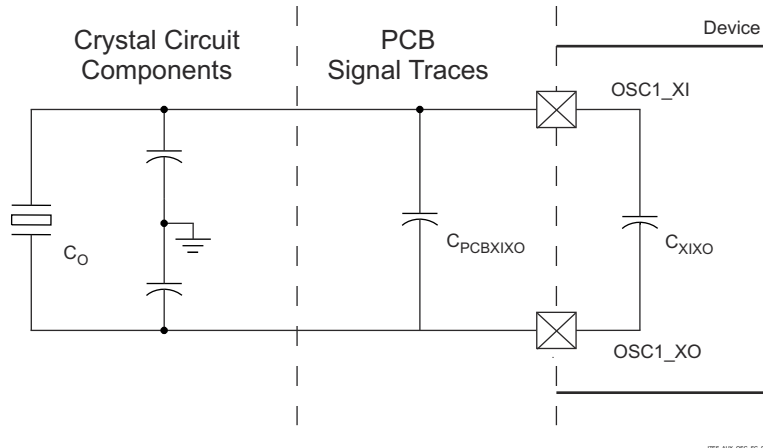
图 8-22. Shunt Capacitance
