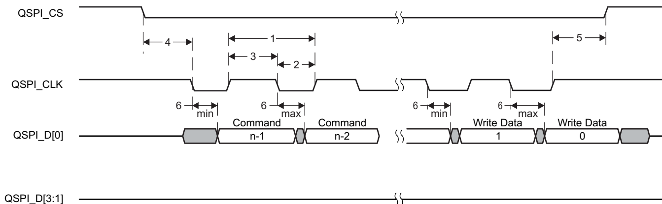
图 5-102. QSPI Write Active High Polarity
