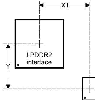
图 5-81. Placement Specifications
