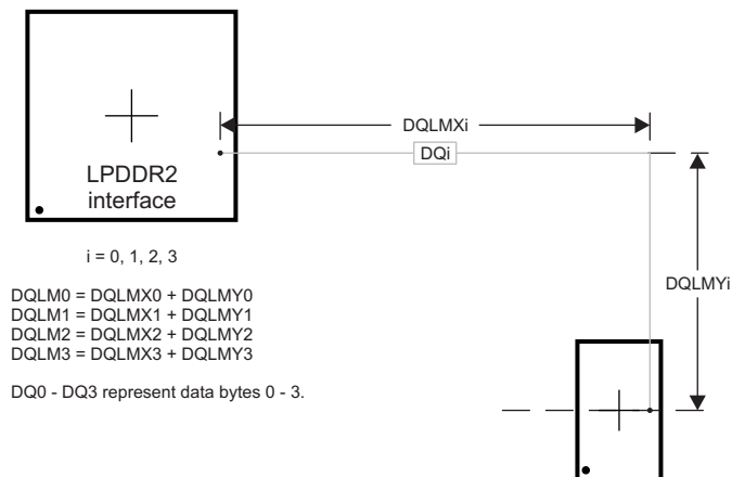
图 5-86. DQ[x] Routing
