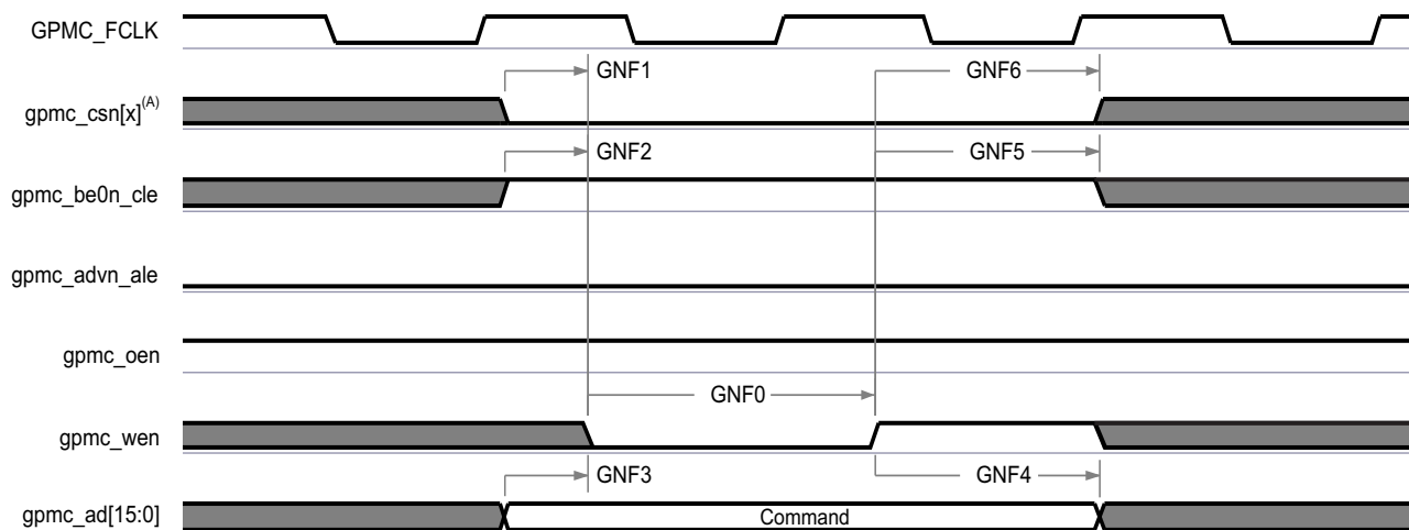
图 5-44. GPMC and NAND Flash—Command Latch Cycle
