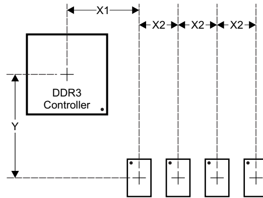
图 5-54. Placement Specifications
