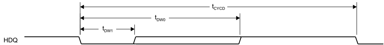
图 5-105. HDQ Write Bit Timing (Command/Address or Data)
