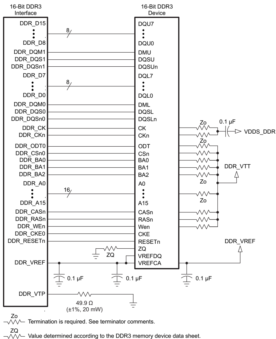
图 5-49. 16-Bit DDR3 Interface Using One 16-Bit DDR3 Device With V_{\text{TT}} Termination
