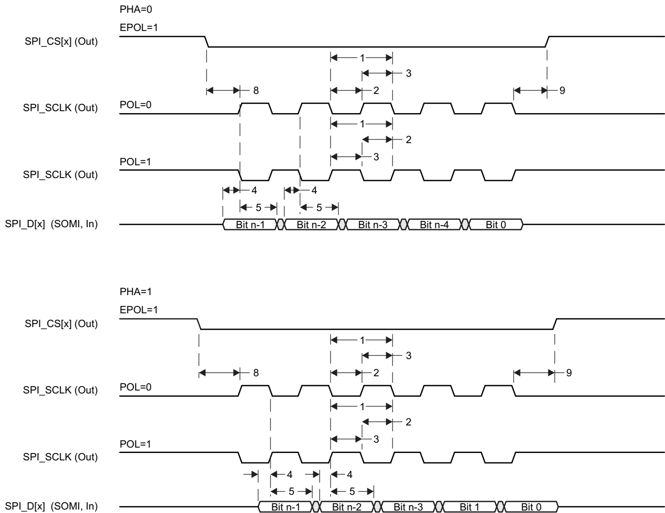
图 5-99. SPI Master Mode Receive Timing
