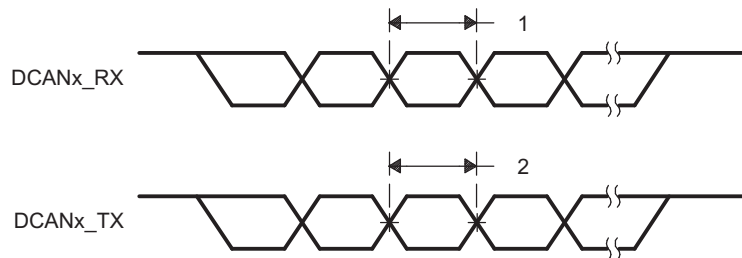
图 5-17. DCANx Timings
