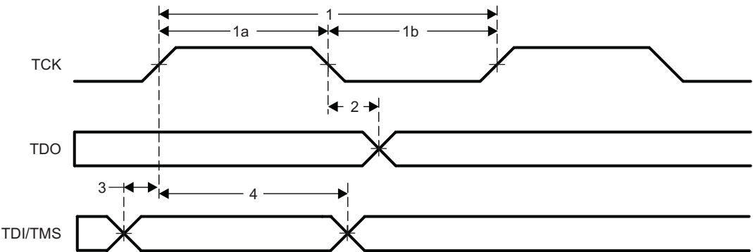
图 5-137. JTAG Timing
