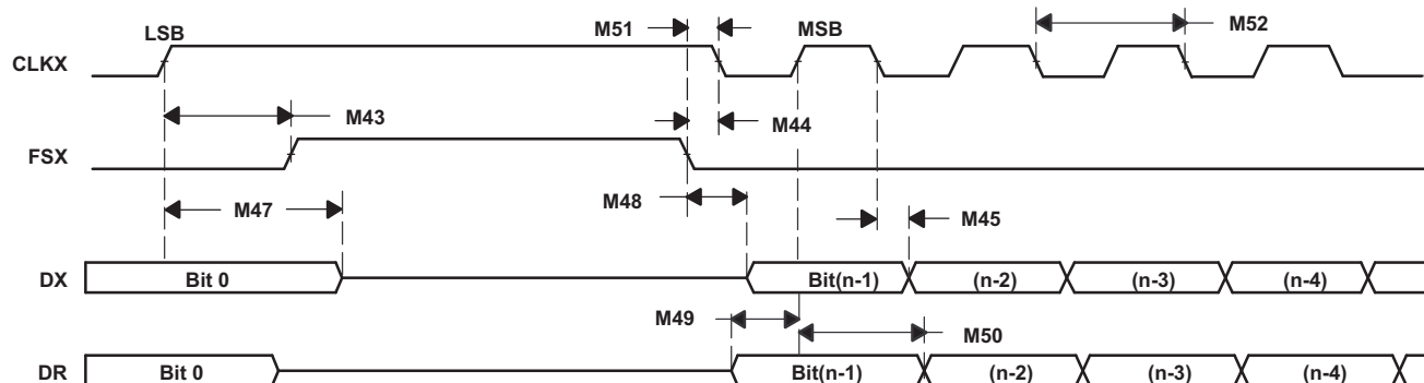
图 5-63. McBSP Timing as SPI Master or Slave: CLKSTP = 10b, CLKXP = 1
