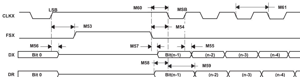
图 5-64. McBSP Timing as SPI Master or Slave: CLKSTP = 11b, CLKXP = 1
