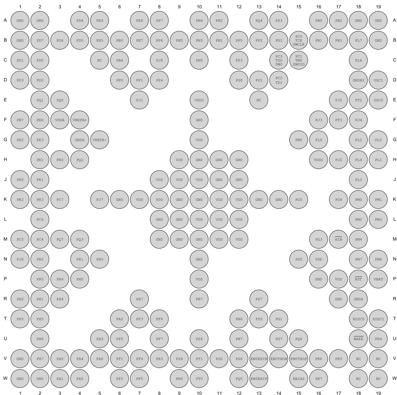
图 4-1. 212-Pin ZAD Package (Top View)
