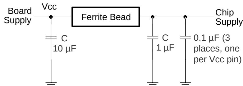
Figure 20. Power-Supply Decoupling
