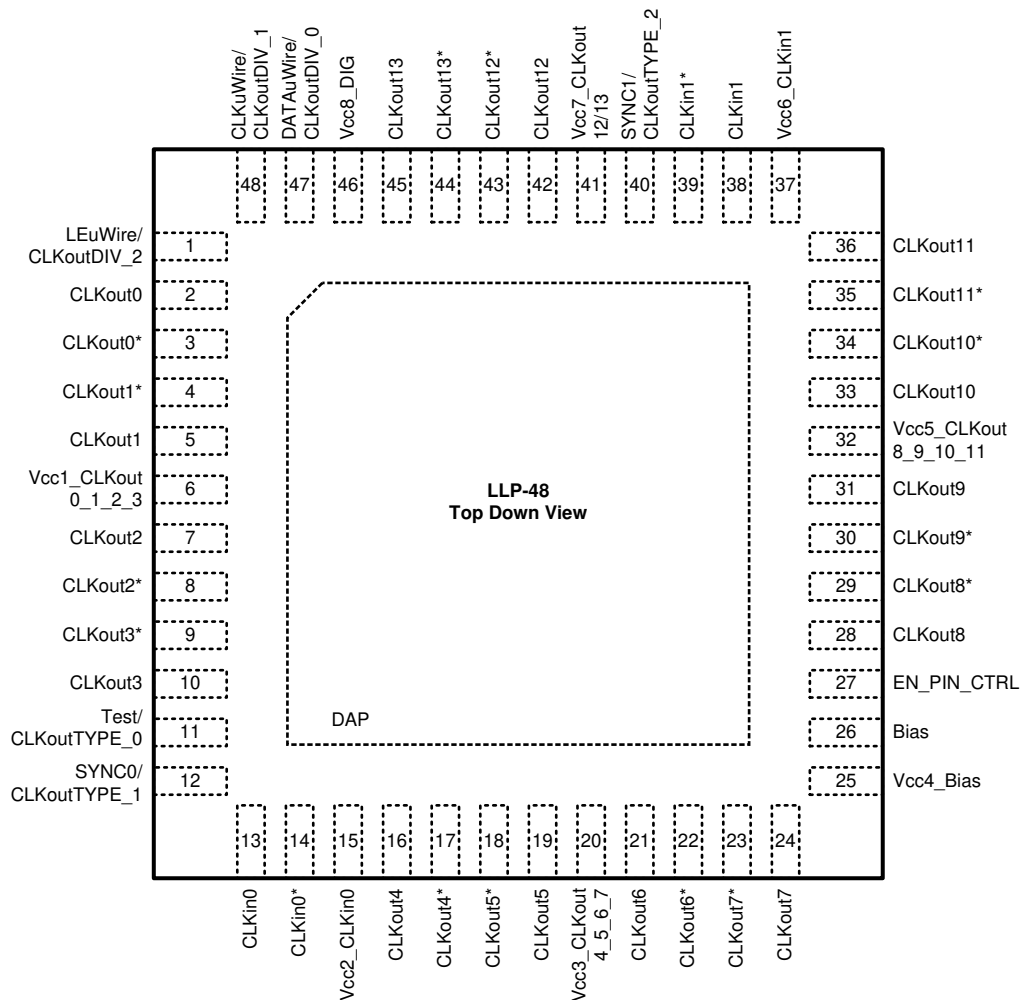
Figure 4-1. 48-Pin Package
