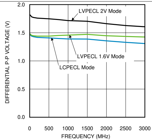
See Section 6.1 for a description of V_{SS} . Figure 5-3. LVPECL V_{SS} vs. Frequency
