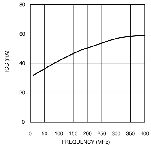
Figure 5-5. Typical Dynamic I_{CC} , C_L = 5 pF
