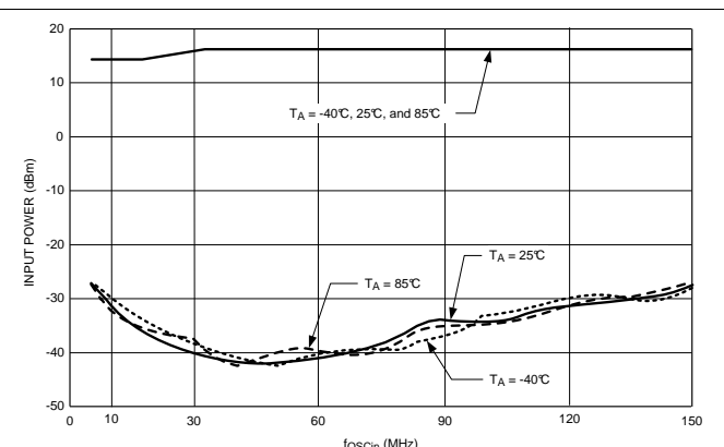
Figure 7. OSCin Sensitivity
