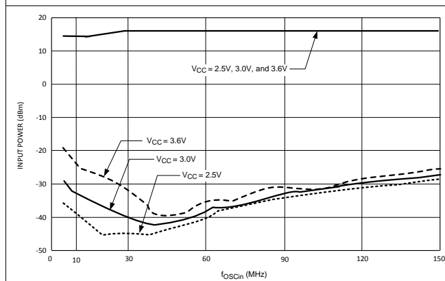
Figure 6. OSCin Sensitivity
