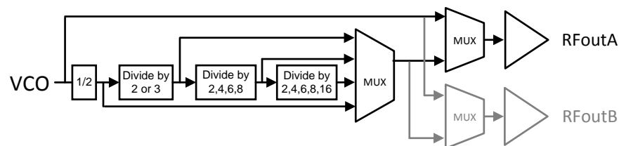
Figure 30. Channel Divider
