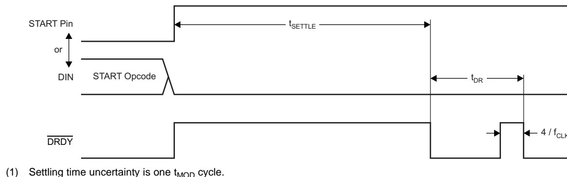
Figure 48. Settling Time
