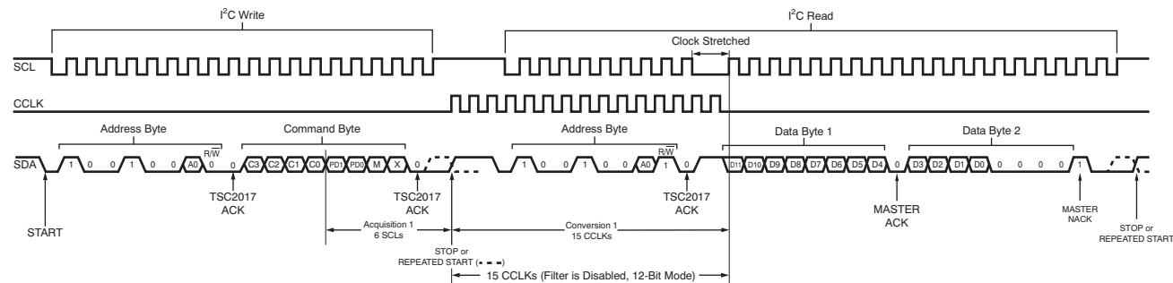
Figure 34. Data Acquisition Cycle (Filter Disabled)
