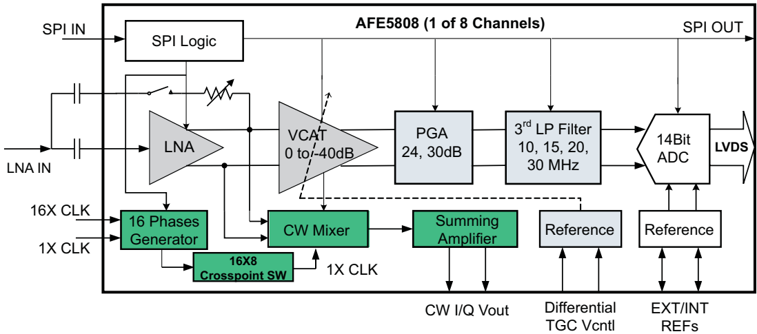
Figure 1. Block Diagram
