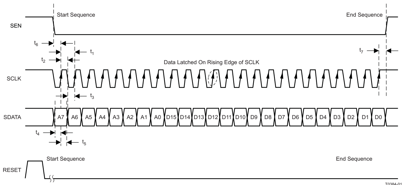
Figure 59. SPI Timing
