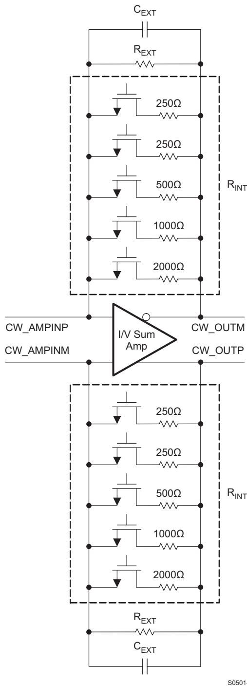
Figure 86. CW Summing Amplifier Block Diagram
