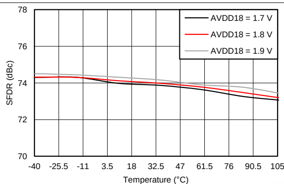
Figure 25. Spurious-Free Dynamic Range vs AVDD18 and Temperature (PGA Gain = 0\text{ dB} , Default Mode)
