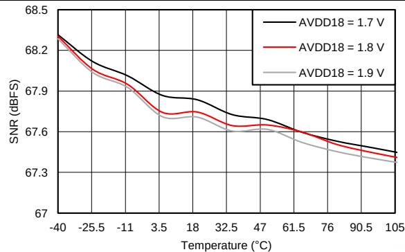
Figure 23. Signal-to-Noise Ratio vs AVDD18 and Temperature (PGA Gain = 0\text{ dB} )
