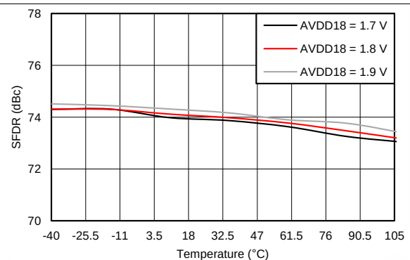
Figure 26. Spurious-Free Dynamic Range vs AVDD18 and Temperature (PGA Gain = 30\text{ dB} , Default Mode)
