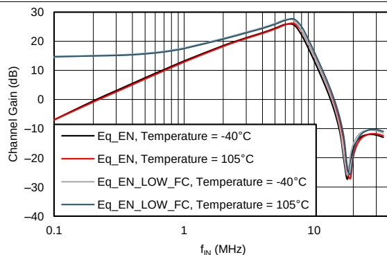
Figure 44. Antialias Filter Response for Equalizer Modes (PGA Gain = 0\text{ dB} )
