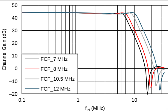
Figure 41. Antialias Filter Response vs FILTER_BW Settings (PGA Gain = 30\text{ dB} )
