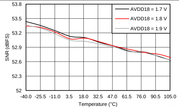
Figure 24. Signal-to-Noise Ratio vs AVDD18 and Temperature (PGA Gain = 30\text{ dB} )
