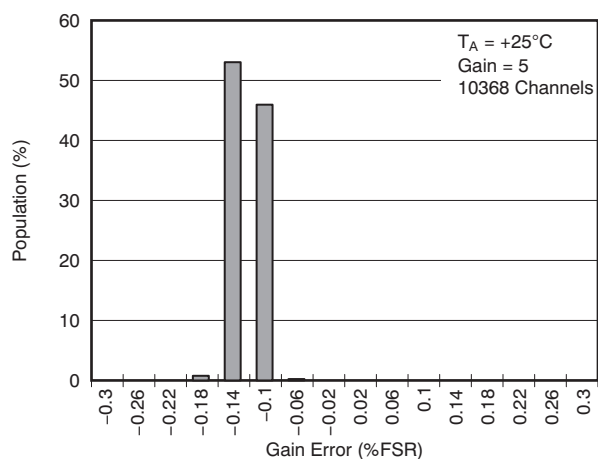
Figure 21. GAIN ERROR
