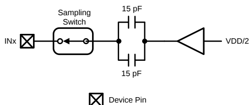
Figure 15. ADC Sampling when AREF is Externally Supplied
