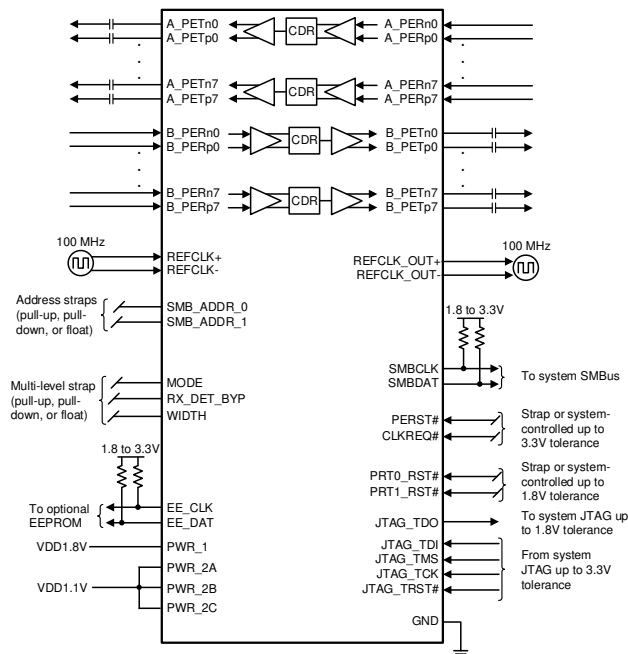
Simplified Schematic
